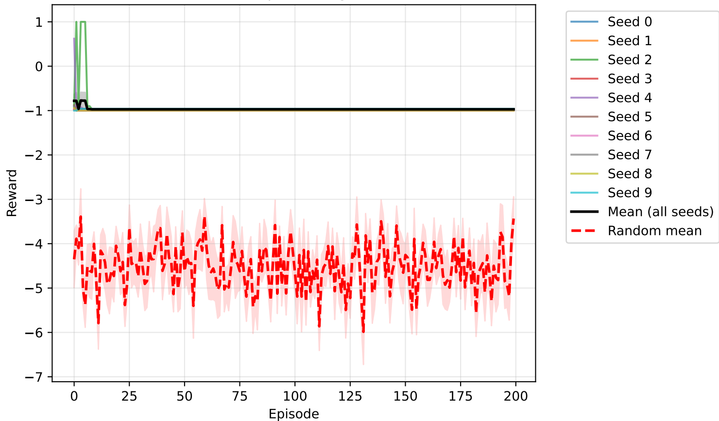
REINFORCE Reward vs Episodes (gamma=0.99, lr=0.1)
