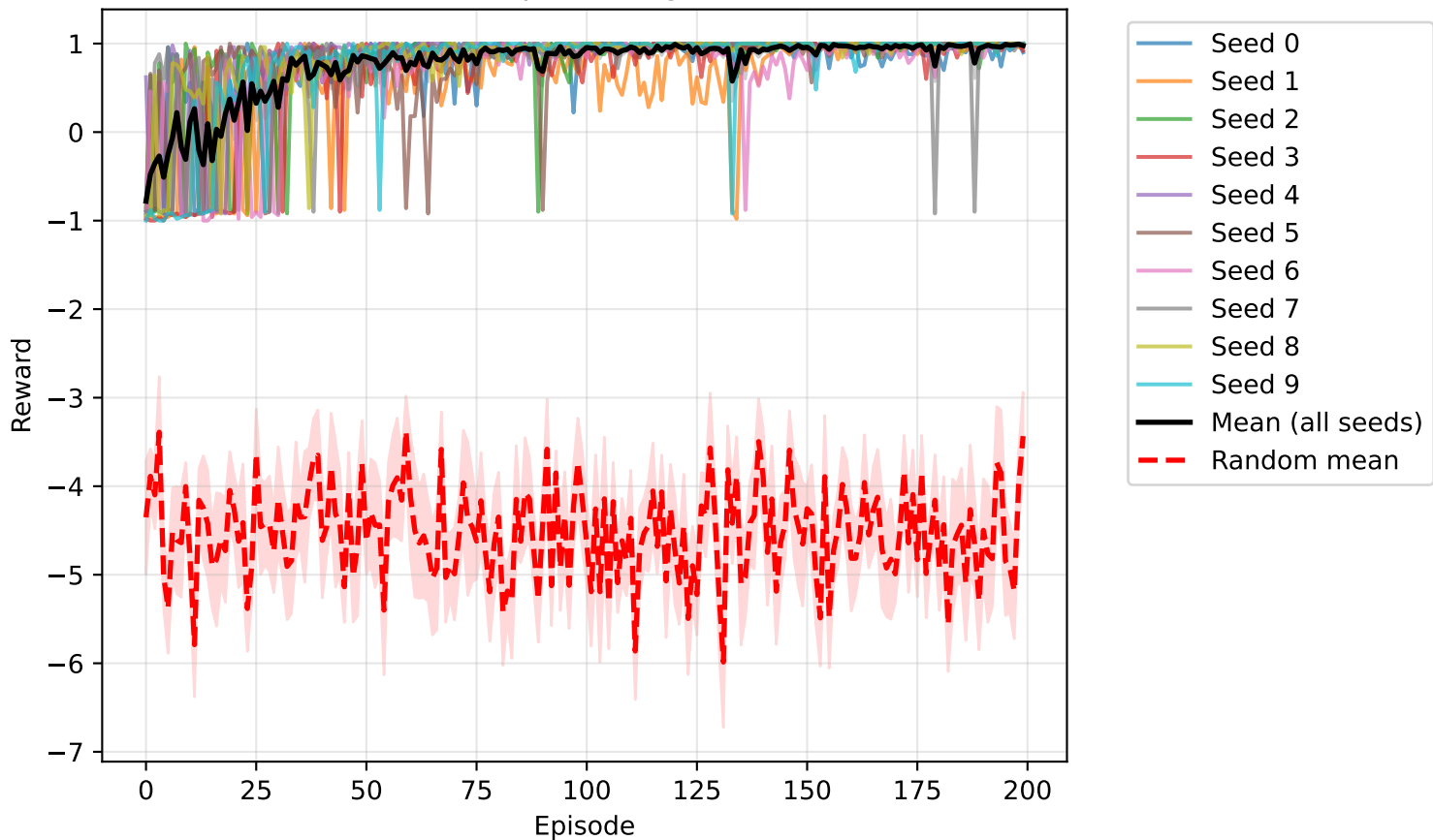
REINFORCE Reward vs Episodes (gamma=0.9, lr=0.001)
