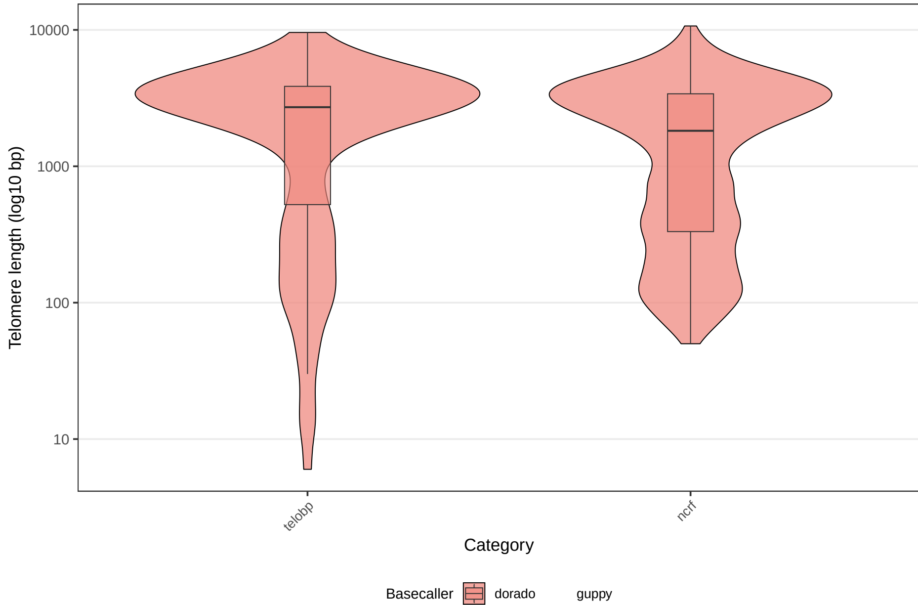
Dorado 1.4.0 SUP – NCRF vs TeloBP (log10 scale)
