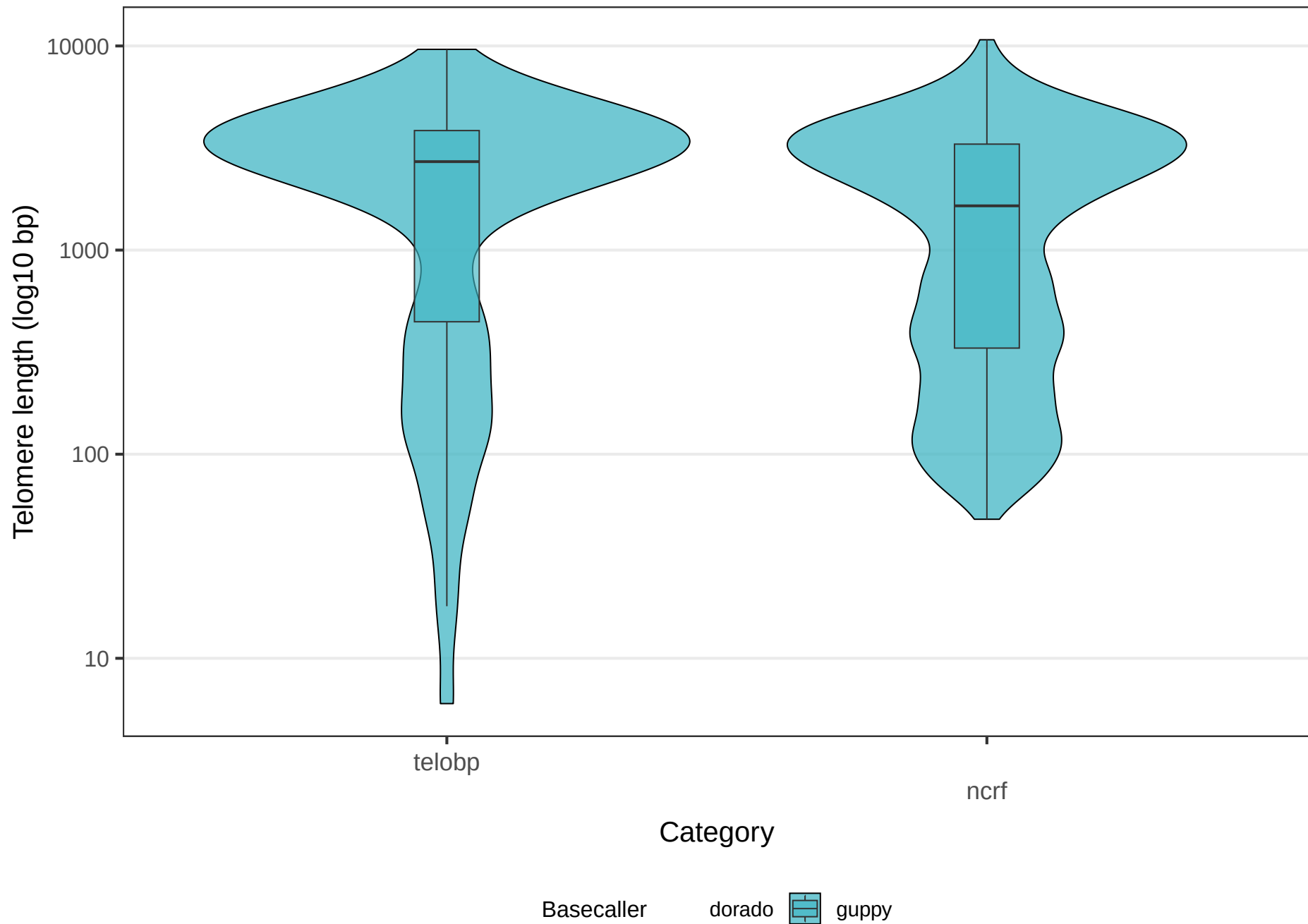
Guppy 6.5.7 SUP – NCRF vs TeloBP (log10 scale)
