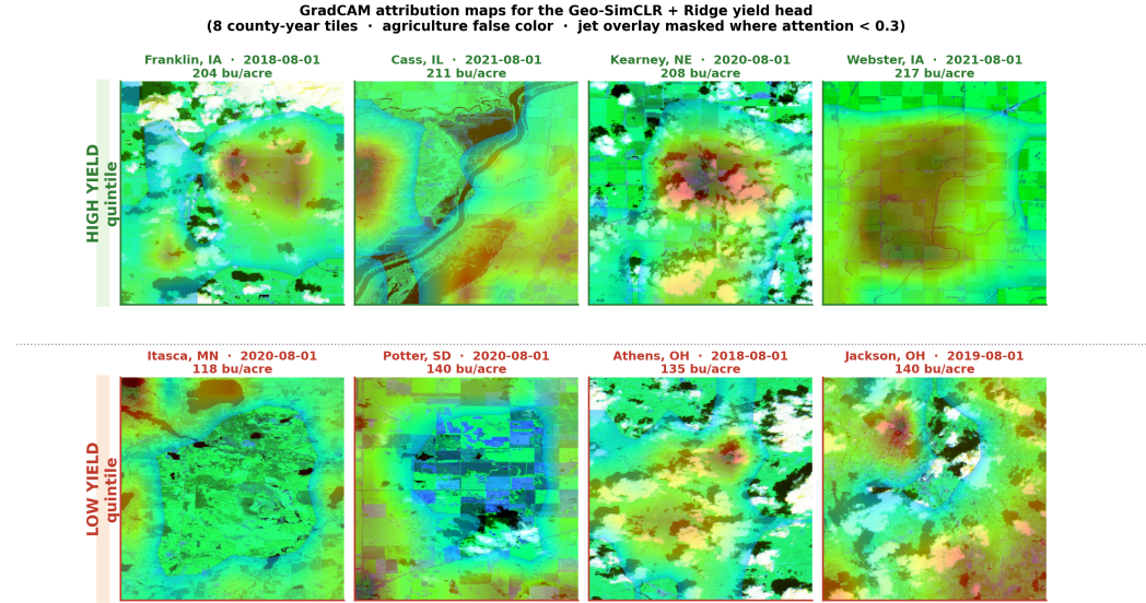
Figure 7: GradCAM [24] attribution maps for the composition of the frozen Geo-SimCLR encoder and a Ridge yield head, computed via Captum’s LayerGradCam [16] on layer4[-1] . Top row: four highest-yield-quintile county-years; bottom row: four lowest. Tiles are rendered in agriculture false-colour with a global 2nd–98th-percentile contrast stretch; the jet overlay is masked to the top 70 % of attention so only high-attention regions are coloured.
