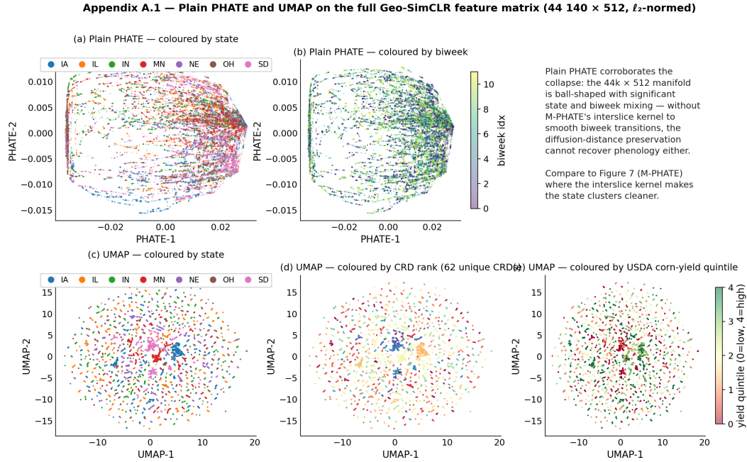
Figure 10: Plain PHATE [20] and UMAP [19] on the same 44,140 \times 512 \ell_2 -normalised feature matrix used for the collapse diagnostic in Section 4.6. (a, b) PHATE coloured by state and biweek; without M-PHATE's inter-slice kernel, the diffusion-distance preservation cannot recover phenology either, and the embedding is ball-shaped with significant state and biweek mixing. (c, d, e) UMAP coloured by state, by Crop Reporting District rank (62 unique CRDs), and by USDA corn-yield quintile. All three views corroborate the SVD-based collapse evidence: the manifold is too dense for UMAP's local-distance focus to find clean state boundaries.
