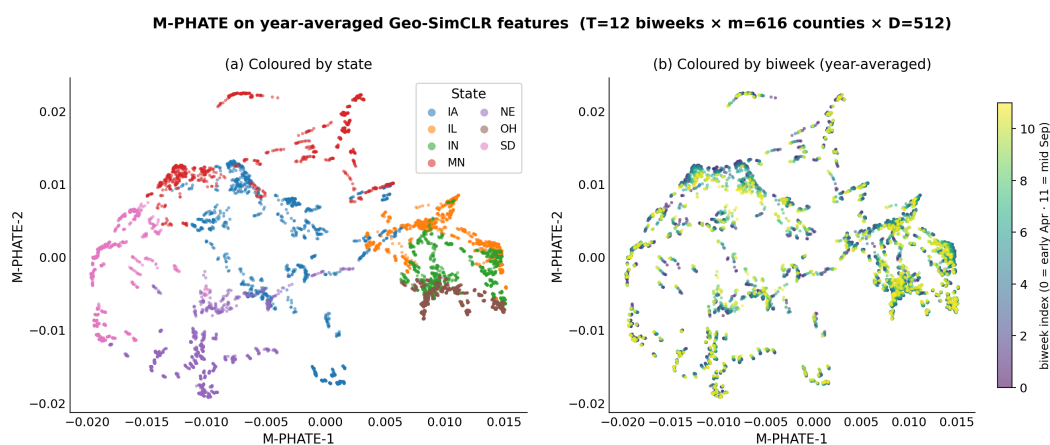
Figure 5: M-PHATE [7] 2-D embedding of Geo-SimCLR features on the year-averaged tensor (12 biweeks \times 616 counties \times 512 features), with intra-slice k = 5 and inter-slice k = 6 neighbour kernels. (a) Coloured by state: state-coherent clusters separate cleanly. (b) Coloured by biweek index: biweek transitions are smooth but tightly overlapping within each state cluster, indicating that seasonal phenology is only weakly encoded relative to geographic identity. M-PHATE’s inter-slice kernel imposes some temporal coherence by construction, so this is a generous upper bound on what the encoder learned about phenology.
