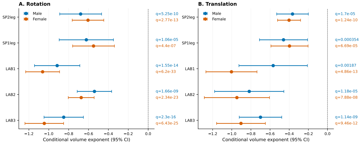
Figure 7: Conditional log-volume slopes. Male and female exponents with HC3 95% CIs from the same adjusted log-log models as Table 4. The vertical zero line indicates no conditional association. Confidence intervals are pointwise; labels give slope q values from the 20-test family. Raw scatterplots and adjusted conditional geometric-mean curves are supplied as Supplementary Figure S1.
