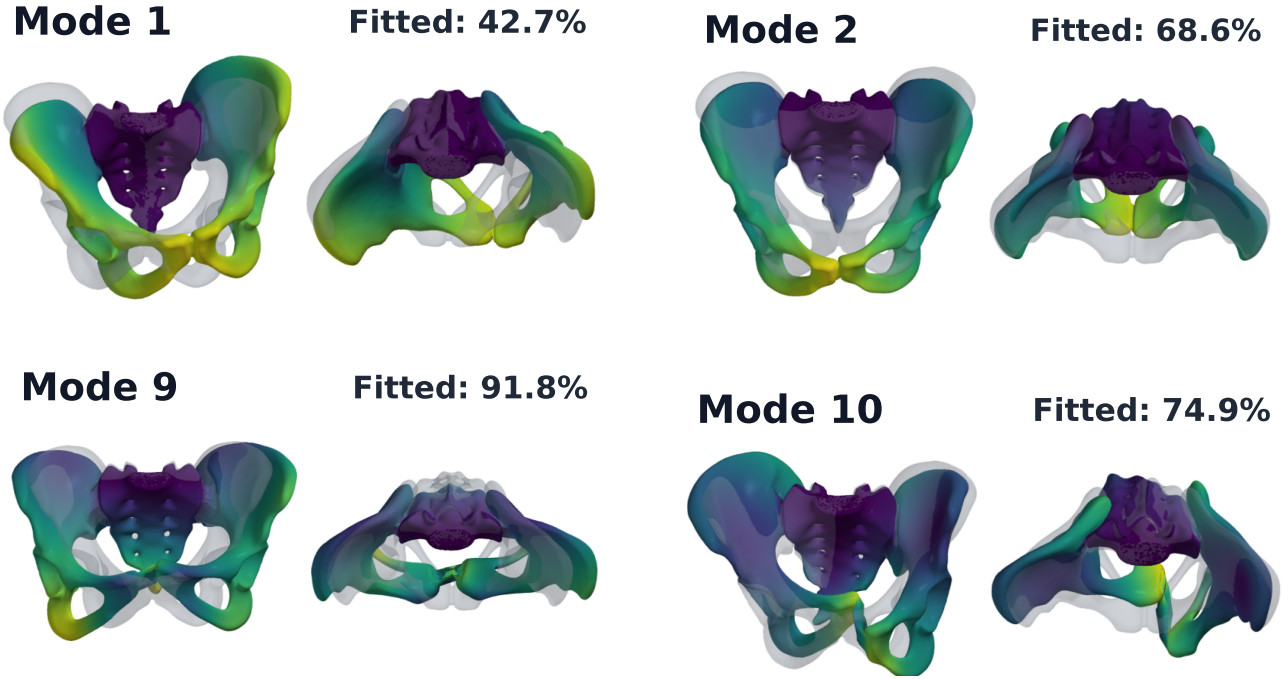
Fig. 2 Low-rank and higher-rank deformation in the single reference pelvis. Existing panels from the complete reference atlas (Appendix A) show modes 1 and 2 above modes 9 and 10. Each panel shows anterior (left) and cranial (right) views; grey is the undeformed geometry and colour indicates relative displacement magnitude. Displacement is enlarged for visualisation to a maximum of 50 mm in every panel. The indicated nonrigid percentages (3.3%, 5.5%, 92.1%, and 95.7%, respectively) are fractions of total squared displacement norm after infinitesimal whole-pelvis rigid-motion projection, not strain or modal-energy fractions. Decomposition methods and the full 15-mode atlas remain in Appendix A.
