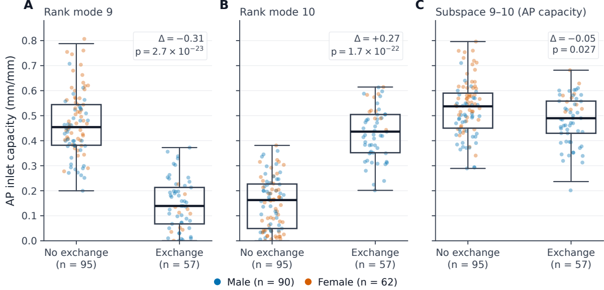
Figure 4: Inlet coupling redistributes between rank labels within the stable 9–10 subspace. Anteroposterior (AP) inlet coupling for rank mode 9 (A), rank mode 10 (B), and the basis-invariant single-functional AP capacity of the two-dimensional 9–10 subspace (C), stratified by 9 \rightleftharpoons 10 label-exchange status. Points represent individual cluster-member subjects ( n=152 ; no-exchange n=95 , exchange n=57 ; male in blue, n=90 ; female in yellow, n=62 ). Horizontal lines indicate medians; boxes indicate interquartile range; whiskers indicate 1.5 \times \text{IQR} . Coupling is expressed as diameter change per millimetre of maximum nodal displacement.
