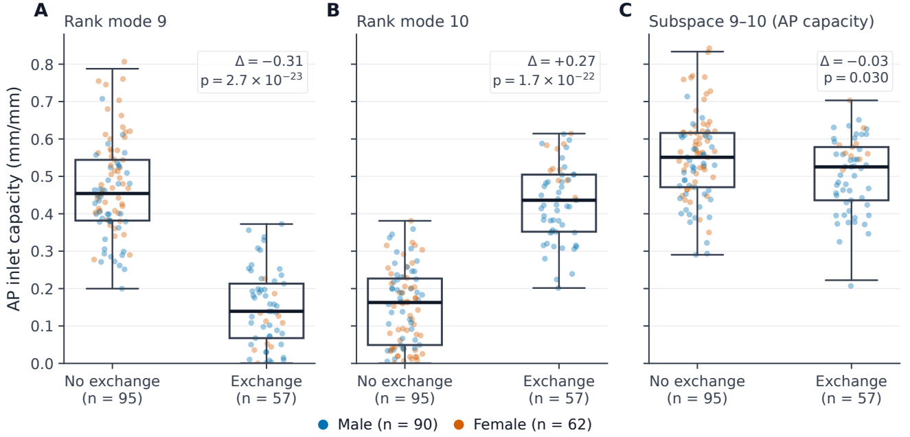
Fig. 5 Inlet coupling redistributes between rank labels within the stable 9–10 subspace. Anteroposterior (AP) inlet coupling for rank mode 9 ( A ), rank mode 10 ( B ), and the basis-invariant single-functional AP capacity of the two-dimensional 9–10 subspace ( C ), stratified by 9 \rightleftharpoons 10 label-exchange status. Points represent individual cluster-member subjects ( n=152 ; no-exchange n=95 , exchange n=57 ; male in blue, n=90 ; female in yellow, n=62 ). Horizontal lines indicate medians; boxes indicate interquartile range; whiskers indicate 1.5 \times \text{IQR} . Coupling is expressed as diameter change per millimetre of maximum nodal displacement.
