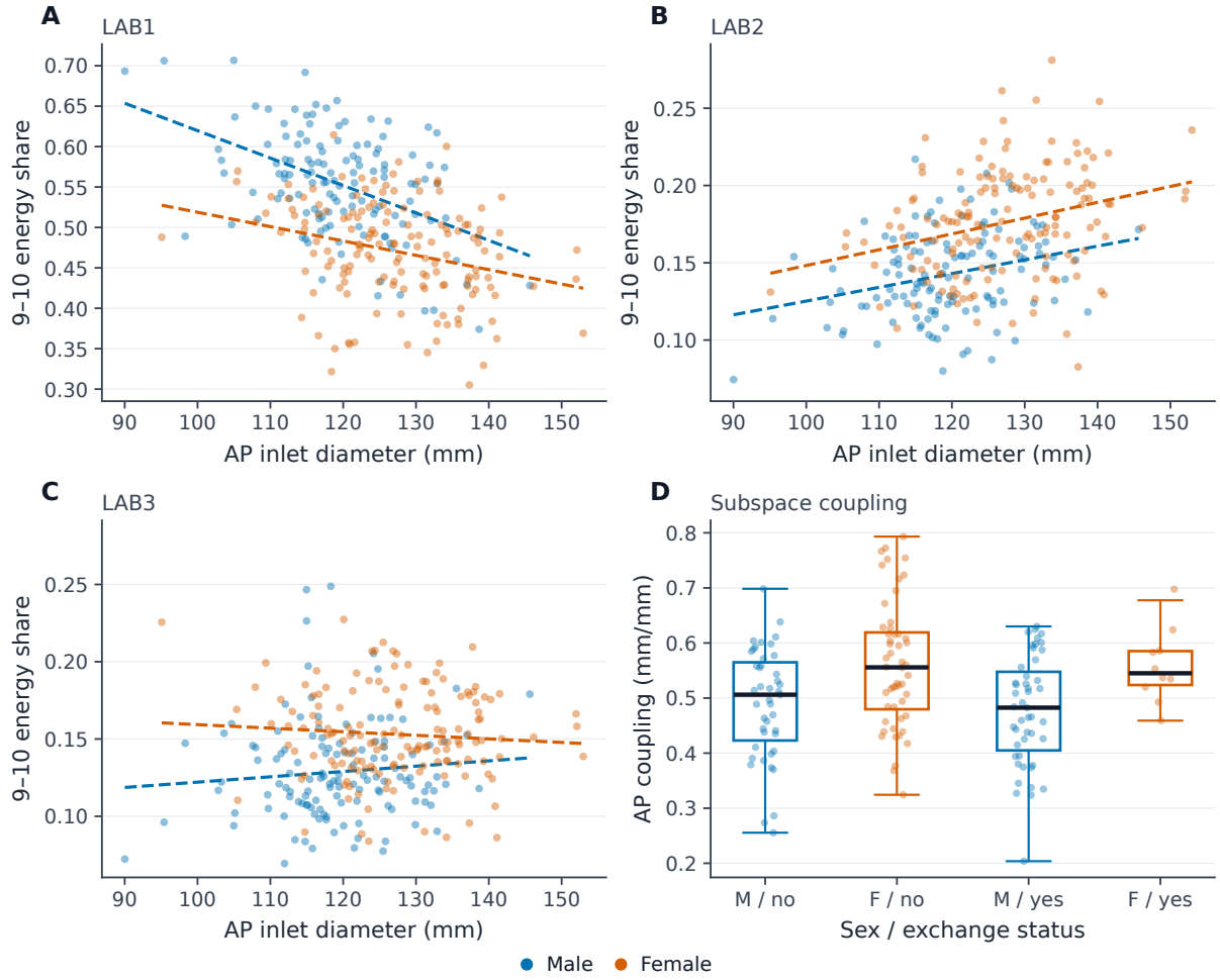
Figure 5: Morphology and loading modulate recruitment of the 9–10 modal block. (A–C) Modal strain-energy fraction carried by the 9–10 block as a function of AP inlet diameter for LAB 1 (bilateral ring compression), LAB 2 (ischial distraction), and LAB 3 (outlet distraction). Blue dots and dashed lines indicate males; yellow dots and dashed lines indicate females. (D) Canonical AP-inlet coupling of the 9–10 subspace stratified jointly by sex and label-exchange status (M/no, F/no, M/yes, F/yes). Boxes show median and IQR; whiskers extend to 1.5 \times \text{IQR} .
