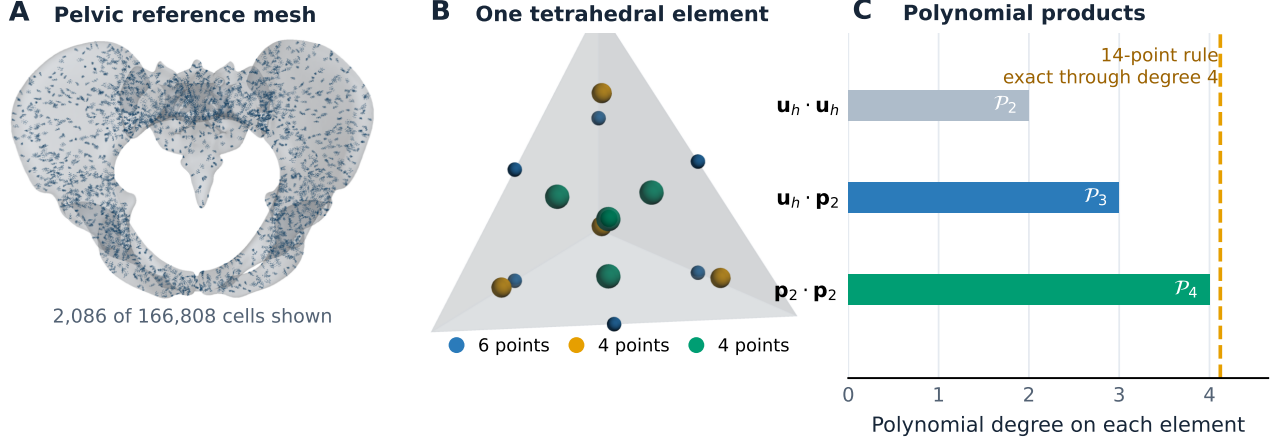
Fig. 2 Volume quadrature for the whole-pelvis displacement decomposition. (A) Reference pelvic mesh with quadrature points displayed for every 80th tetrahedron; the calculation includes all 166 808 cells. (B) The 14 integration points on a standard tetrahedron. Colour and sphere size distinguish the three groups of positive weights (six, four, and four points). The rule is mapped to every tetrahedron in the mesh. (C) Polynomial degrees of the squared P_1 FE displacement, its cross-product with a quadratic dictionary field, and the quadratic dictionary Gram product. The 14-point rule is exact through degree 4 on each tetrahedron.
