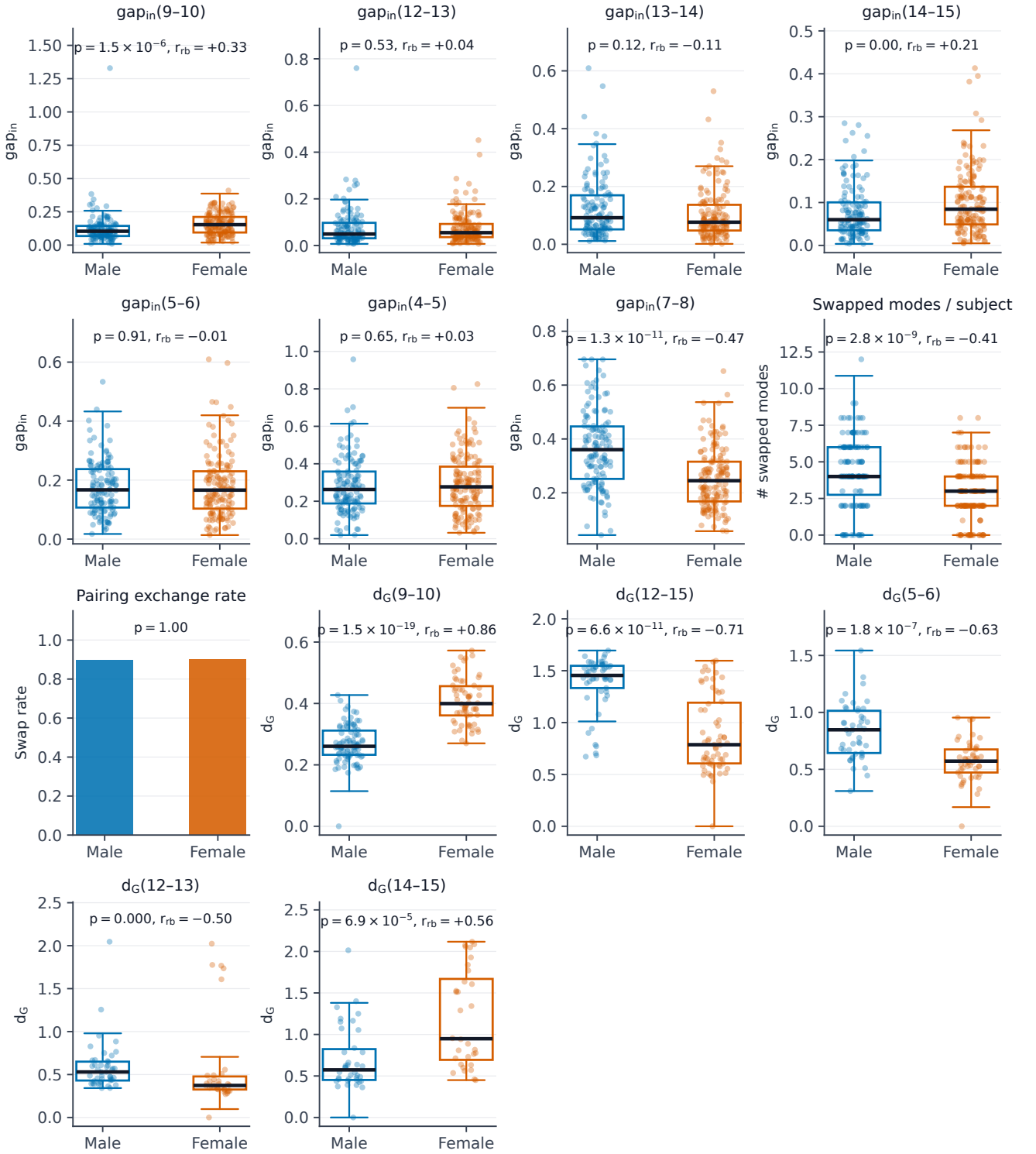
Fig. 5 Sex-stratified spectral summary
