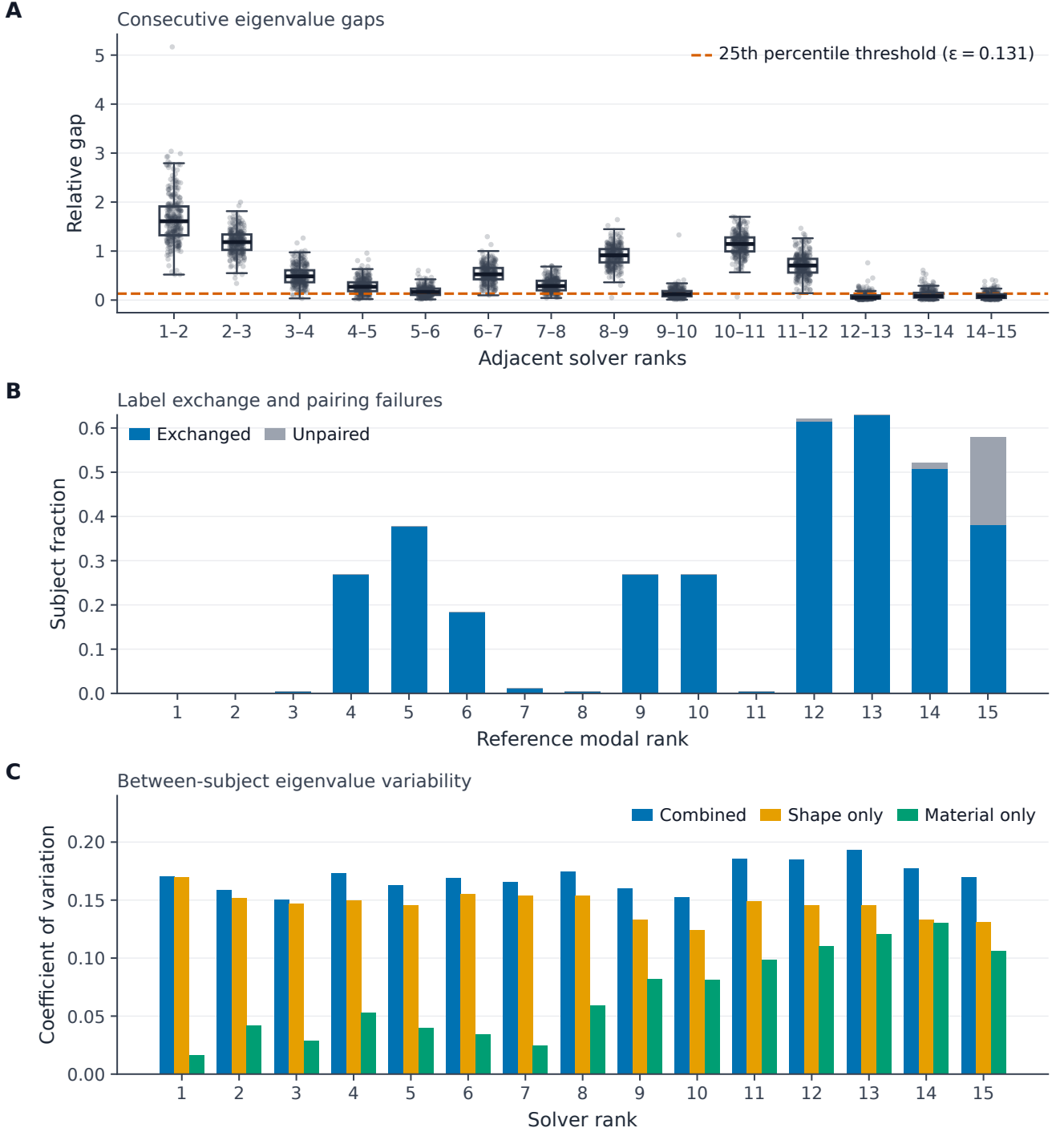
Fig. 2 Population variability partitions the stiffness spectrum into an order-locked backbone and clustered higher ranks. (A) Consecutive relative spectral gaps \text{gap}_{\text{in}}(i) = (\lambda_{i+1} - \lambda_i)/\lambda_i across the cohort ( N=278 ); the dashed line marks the data-driven cluster threshold \epsilon_{\text{in}} \approx 0.131 (25th percentile). (B) Subject fraction exhibiting label exchange (blue) and matches flagged as unpaired (grey; \text{MAC}_{M_{\text{ref}}}^0 < 0.05 ) per reference label. (C) Eigenvalue variability (coefficient of variation, CoV) across the combined cohort (blue), shape-only cohort (orange), and material-only cohort (green).
