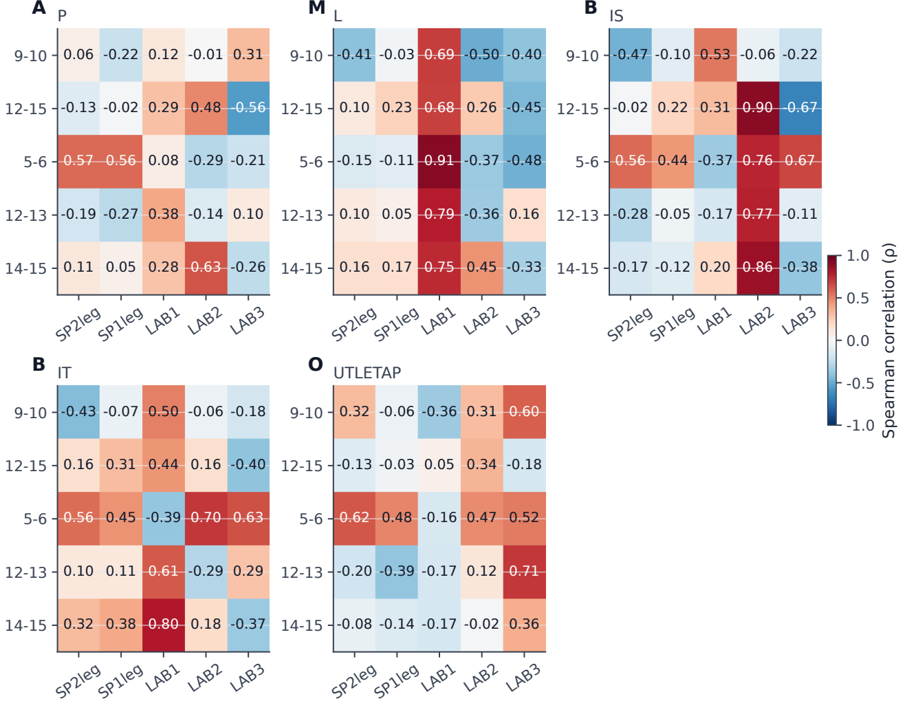
Fig. 12 Exploratory associations between anatomical capacity and load recruitment. Each cell gives the Spearman correlation between the indicated single-functional max-nodal capacity and the block’s retained modal energy fraction among subjects belonging to that rank block. Rows identify the five most prevalent blocks; columns identify the two standing and three comparative expansion loads. The panels correspond to AP and ML inlet, interspinous (BIS), bituberos (BIT), and AP outlet capacity.
