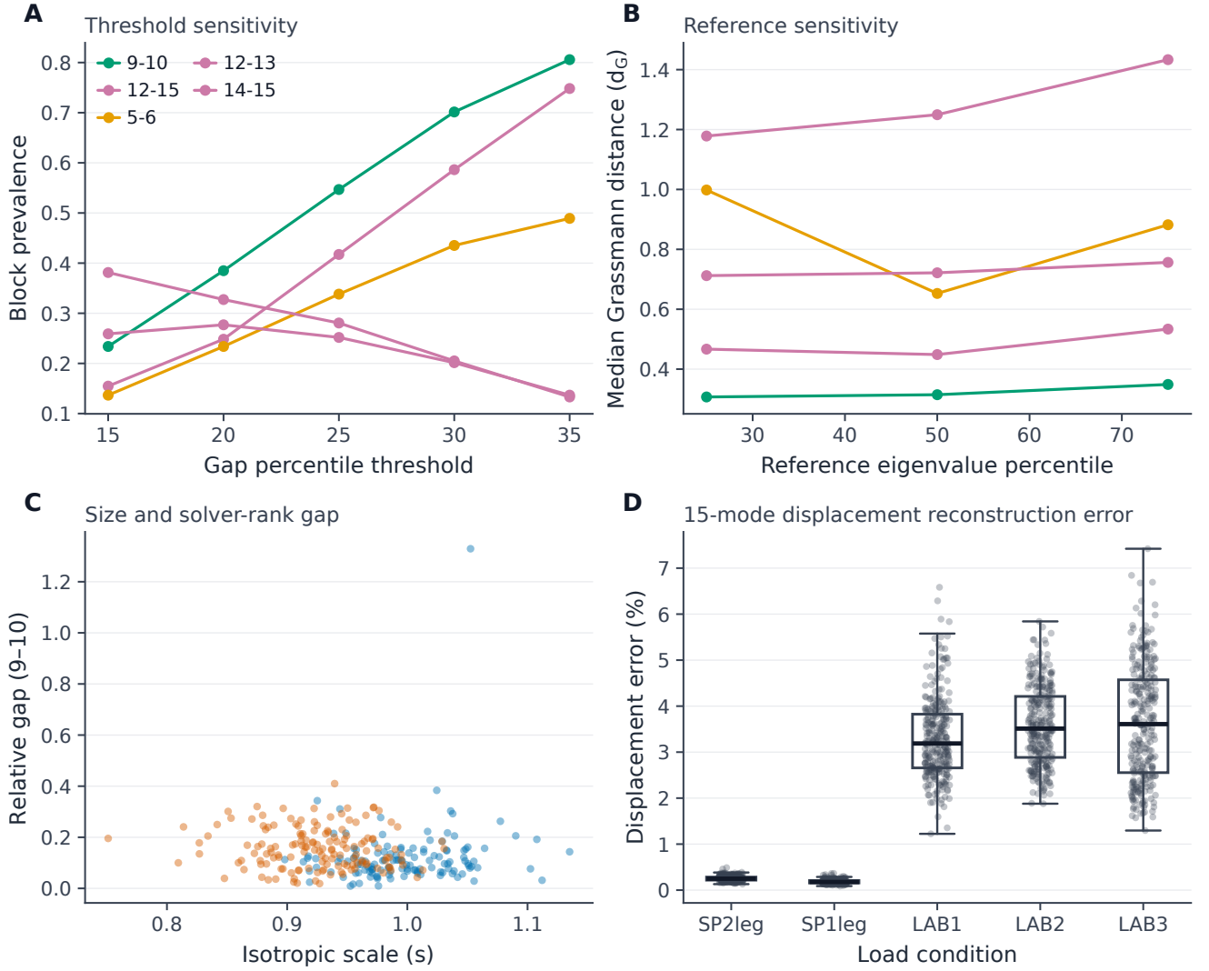
Fig. 8 Robustness and reconstruction dashboard
