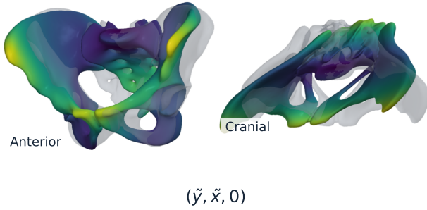
Fig. 10 Representative fields of the 3D polynomial deformation dictionary. One example per family is evaluated on the reference pelvis: (A) axial extension, \mathbf{a}_{x,1} ; (B) shear-free bending, \mathbf{b}_{xy} ; (C) uniform transverse shear, \mathbf{s}_{xy,1} ; and (D) torsion-like twist, \mathbf{t}_x . Each card shows anterior and cranial views. Grey denotes the undeformed geometry; colour indicates displacement magnitude relative to the maximum within that field. The formulas are the raw polynomial dictionary members in dimensionless coordinates, and the rendered fields have their volume-weighted infinitesimal rigid component removed. Each representative basis field is independently scaled to a 50 mm maximum displacement for visibility.
