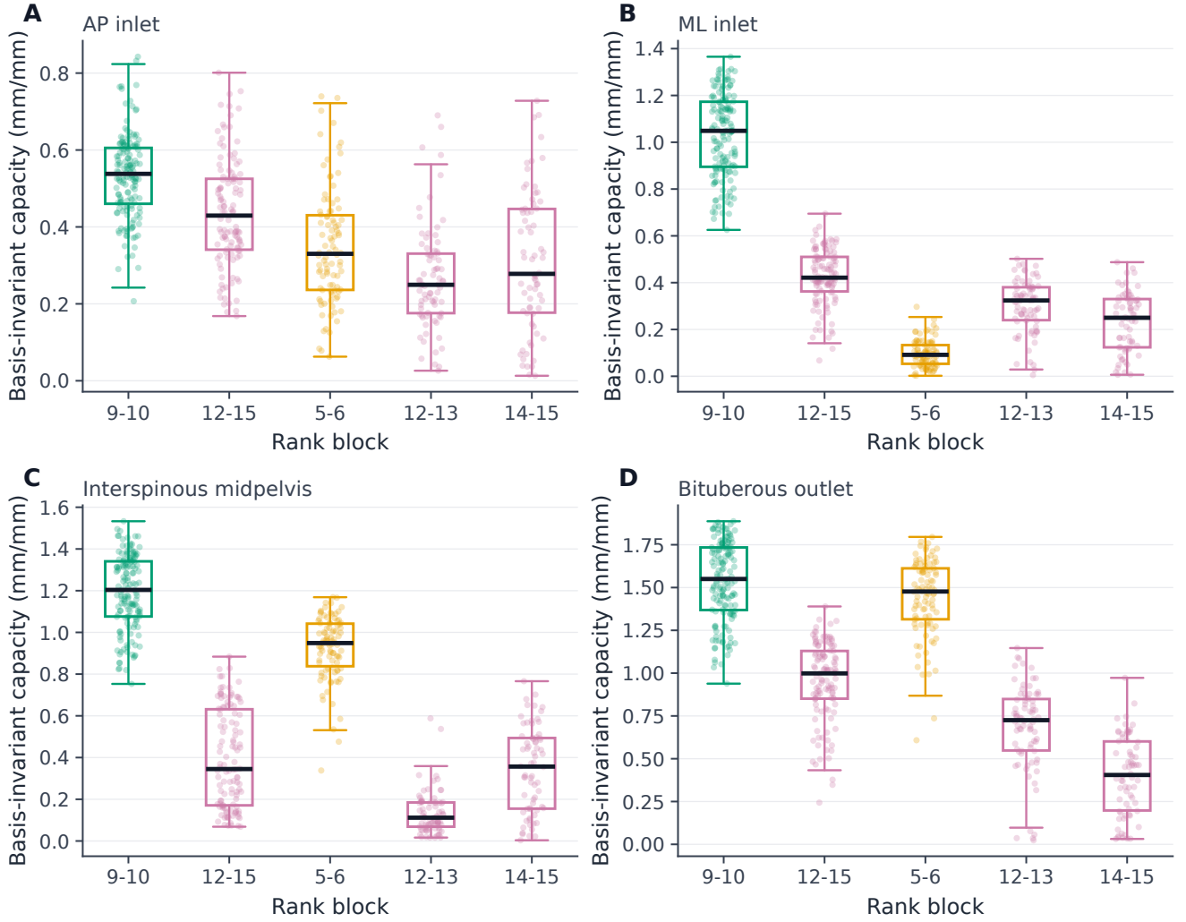
Fig. 3 Basis-invariant anatomical capacities across recurrent clustered modal subspaces. Basis-invariant anatomical capacities (maximum anatomical diameter response per 1 mm maximum nodal displacement) for the five most prevalent rank blocks across the cohort ( N=278 ): (A) anteroposterior (AP) inlet, (B) mediolateral (ML) inlet, (C) interspinous midpelvic diameter, and (D) bituberous outlet. Boxes indicate median and interquartile range (IQR); whiskers extend to 1.5 \times \text{IQR} .
