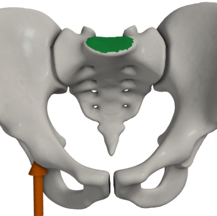
Right acetabular load 800 N total
