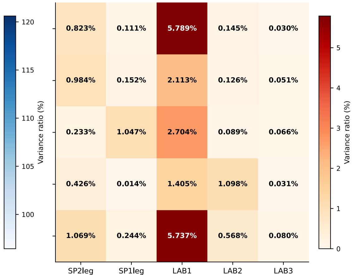
B. Density / template geometry Variance relative to full model (%)
