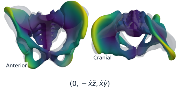
Fig. 3 Representative fields of the 3D polynomial deformation dictionary. One example per family is evaluated on the reference pelvis: (A) axial extension, \mathbf{a}_{x,1} ; (B) shear-free bending, \mathbf{b}_{xy} ; (C) uniform transverse shear, \mathbf{s}_{xy,1} ; and (D) torsion-like twist, \mathbf{t}_x . Each card shows anterior and cranial views. Grey denotes the undeformed geometry; colour indicates displacement magnitude relative to the maximum within that field. The formulas are the raw polynomial dictionary members in dimensionless coordinates, and the rendered fields have their volume-weighted infinitesimal rigid component removed. Each rendered field is independently scaled to 50 mm maximum displacement for visibility; these are illustrative basis fields, not computed FE eigenmodes or predicted load responses.
