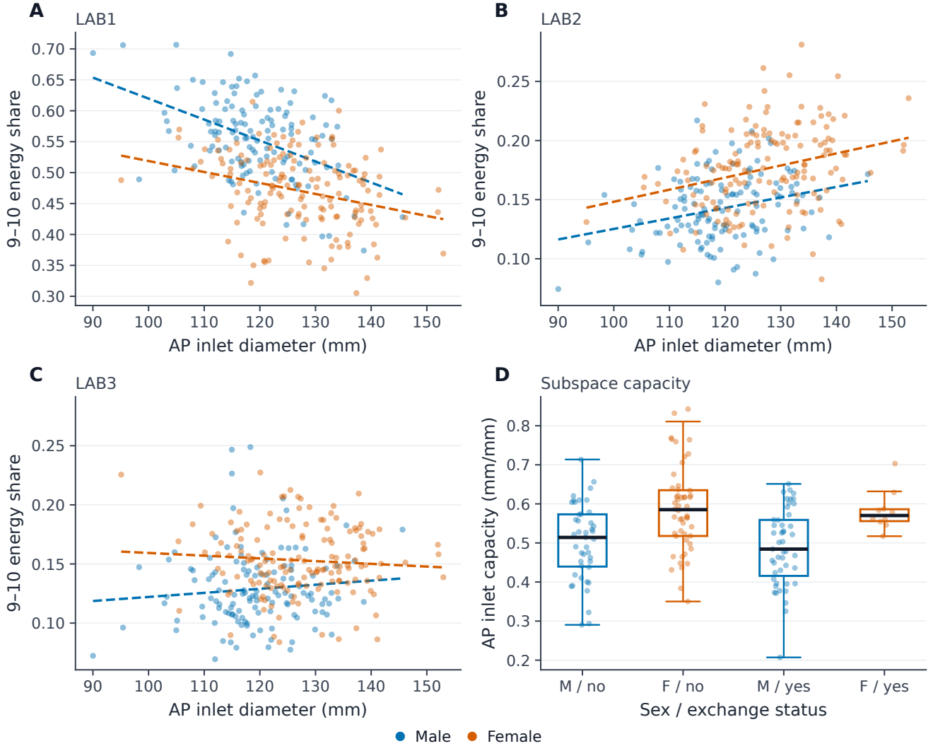
Fig. 11 Morphology and loading modulate recruitment of the 9–10 modal block. (A–C) Modal strain-energy fraction carried by the 9–10 block as a function of AP inlet diameter for LAB 1 (bilateral internal ring expansion), LAB 2 (ischial distraction), and LAB 3 (outlet distraction). Blue dots and dashed lines indicate males; yellow dots and dashed lines indicate females. (D) Basis-invariant single-functional AP-inlet capacity of the 9–10 subspace stratified jointly by sex and label-exchange status (M/no, F/no, M/yes, F/yes). Boxes show median and IQR; whiskers extend to 1.5 \times \text{IQR} .
