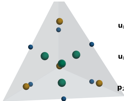
B One tetrahedral element
