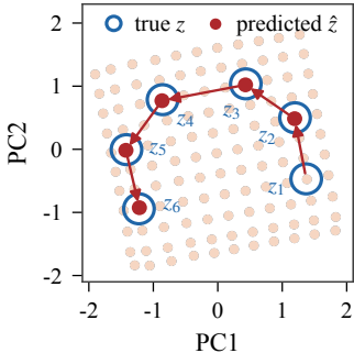
Latent rollout
