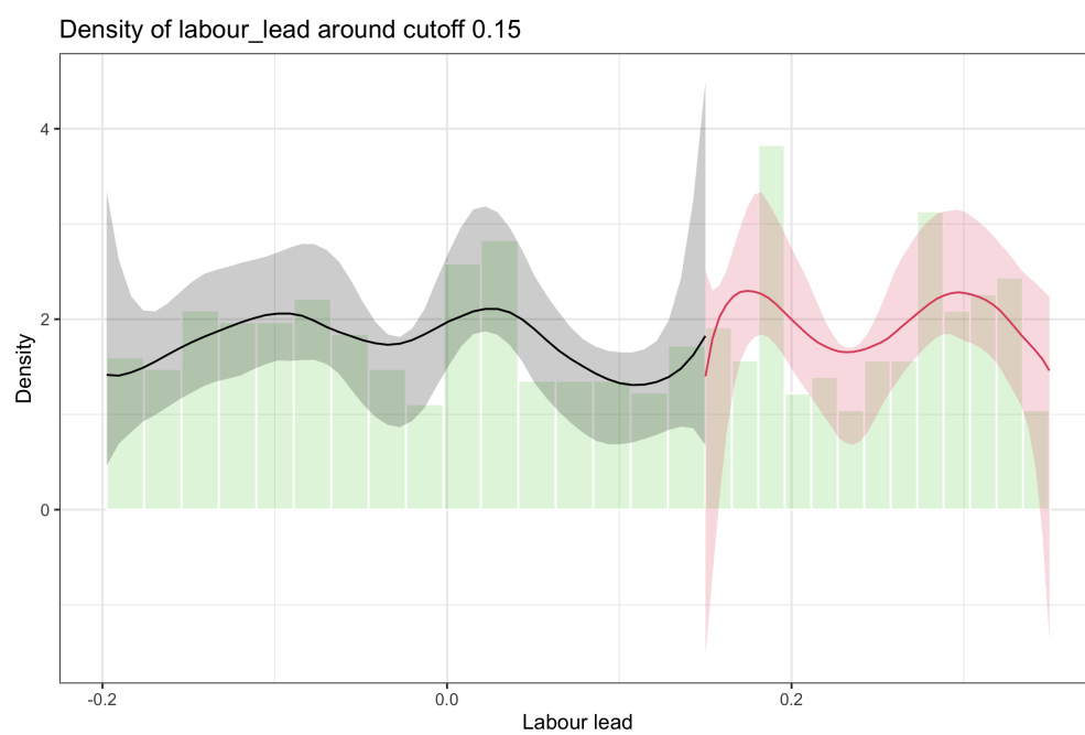
Figure 3: Density discontinuity ( rddensity ) test.
