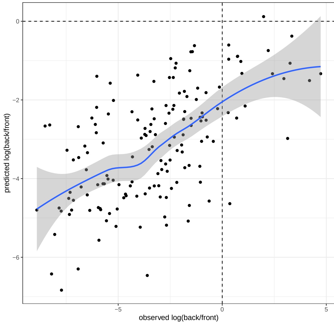
KRR LOO: real words, semantic distance
