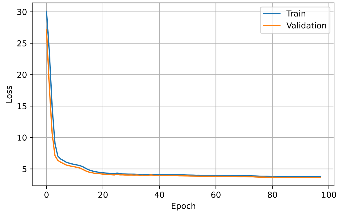
Reconstruction Loss
