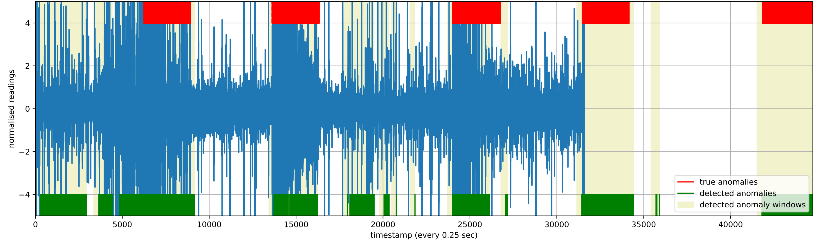
dataset test sequence (normalised by train mean 0.0000 and std 0.0079) Detection method: recon_error_theoretical_best
