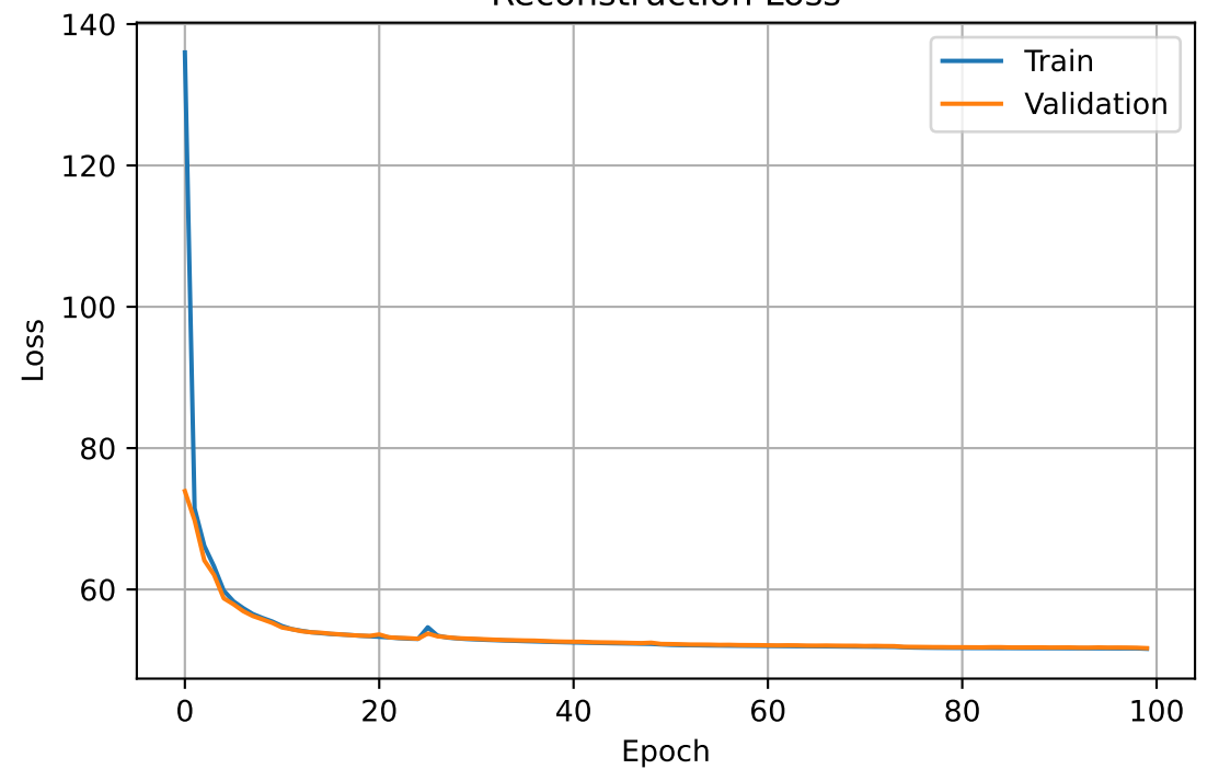
Reconstruction Loss
