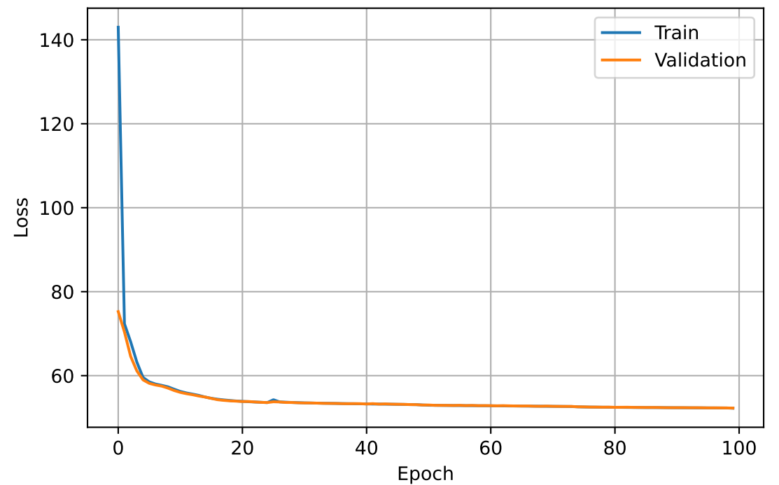
Reconstruction Loss
