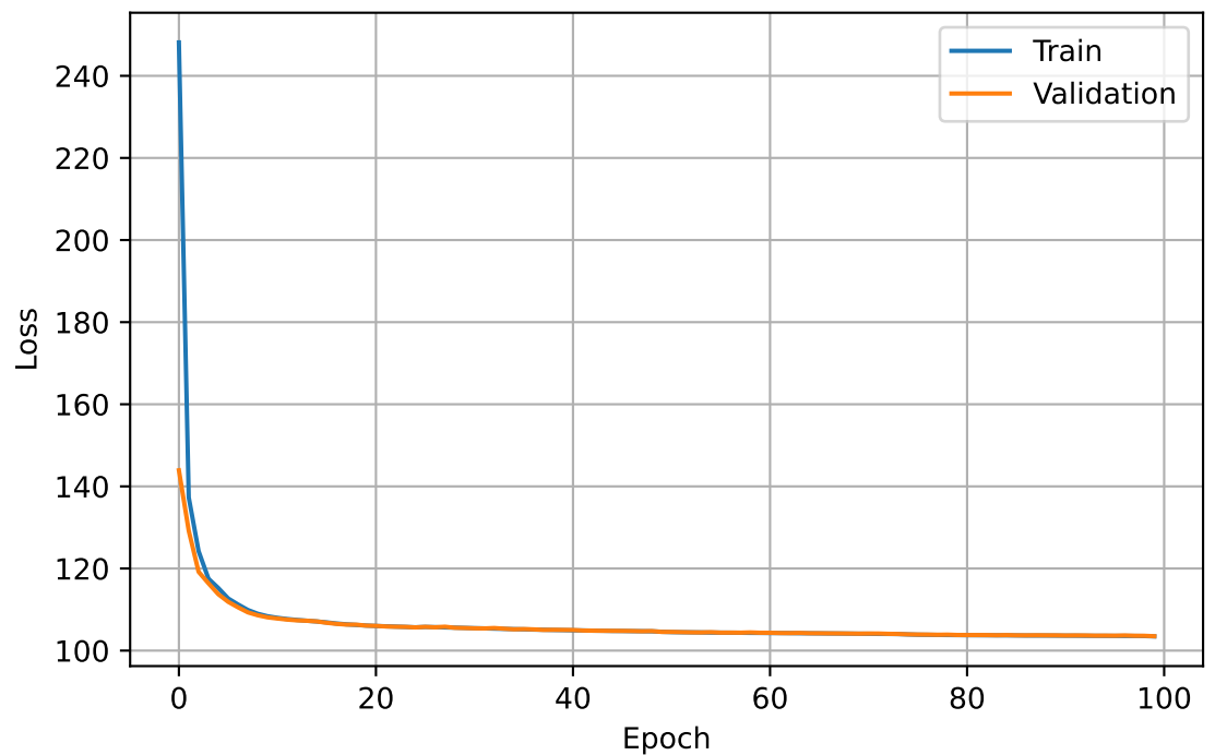
Reconstruction Loss
