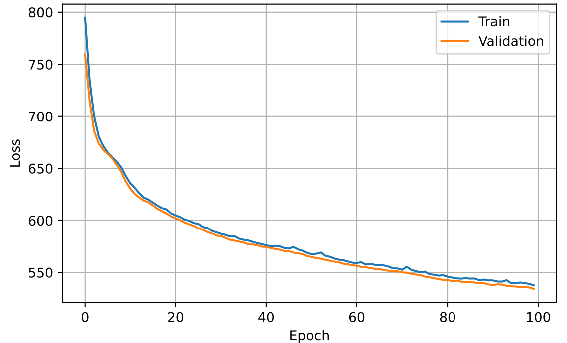
Reconstruction Loss
