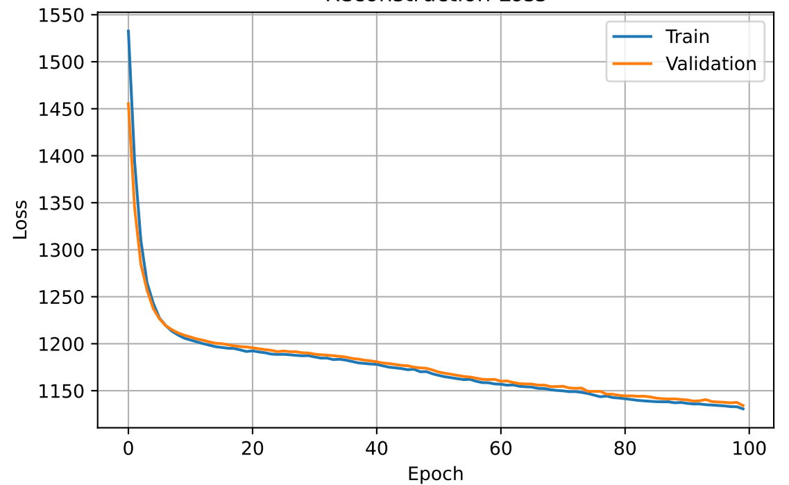
Reconstruction Loss
