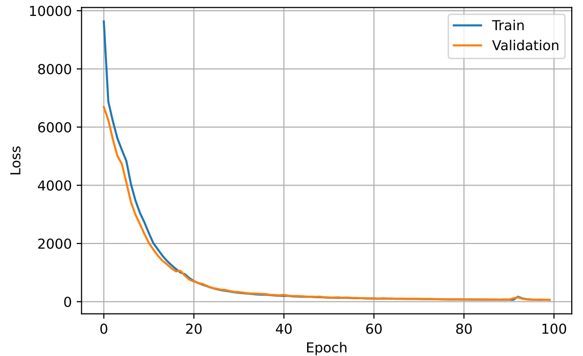
Reconstruction Loss
