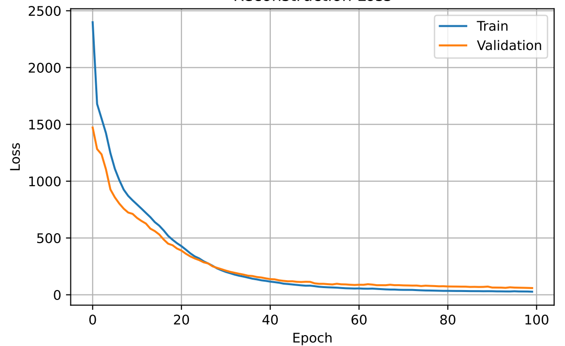
Reconstruction Loss
