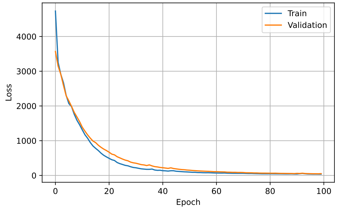
Reconstruction Loss
