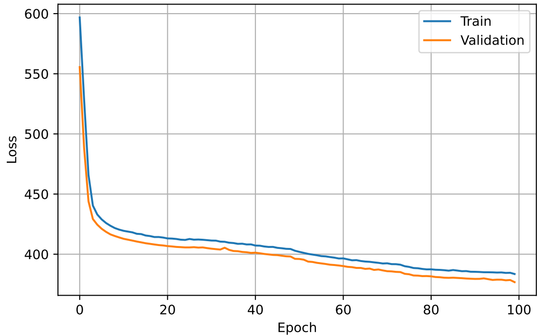
Reconstruction Loss
