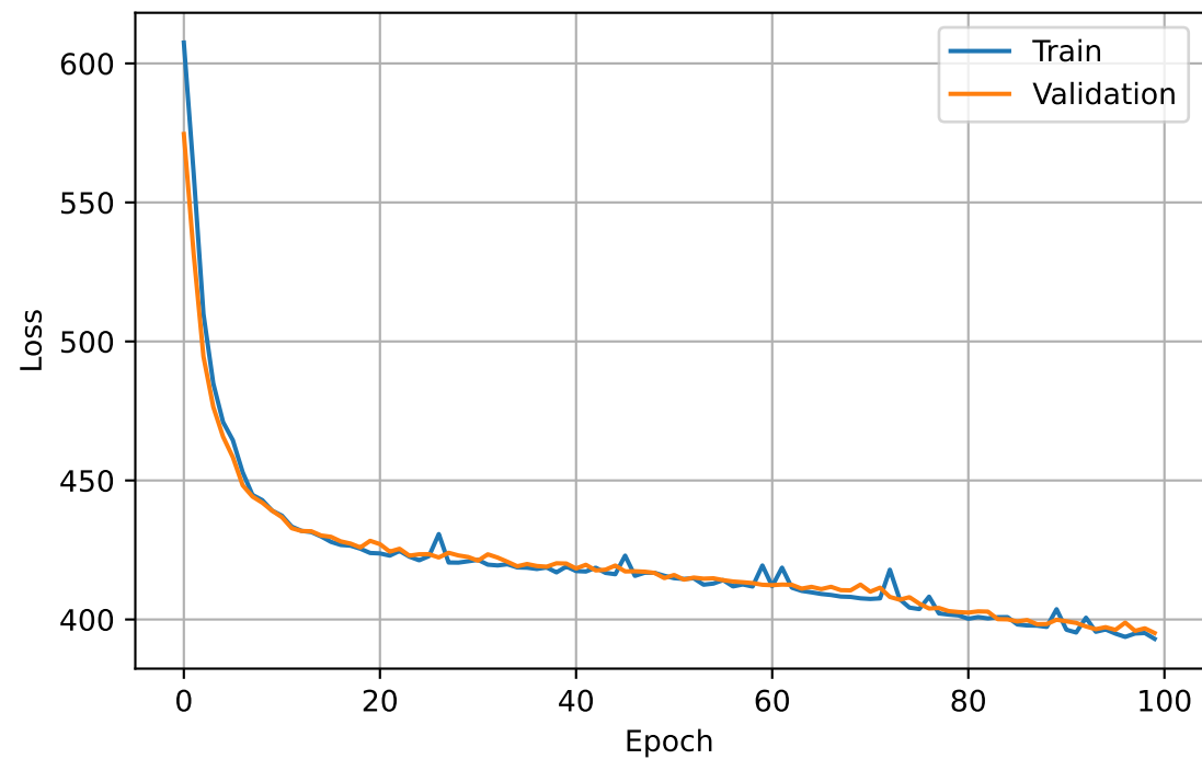
Reconstruction Loss
