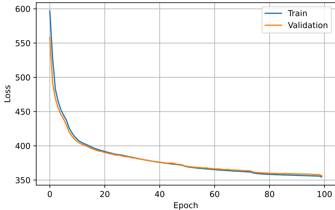
Reconstruction Loss
