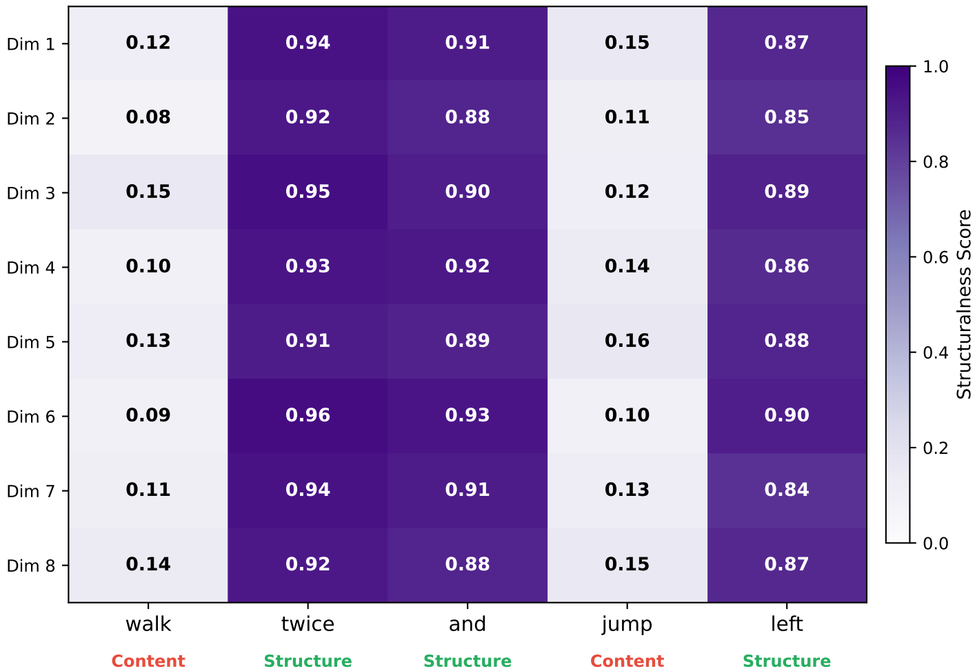
Content words (walk, jump) → Low scores → Suppressed Structural words (twice and left) → High scores → Preserved AbstractionLayer: Structuralness Scores (Higher = More Structural)
