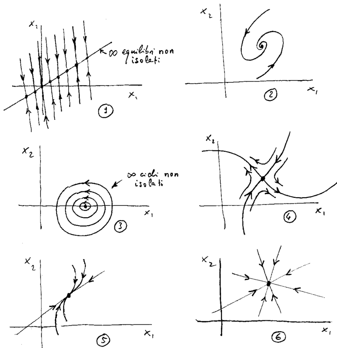
Figure 14.5: Phase portraits
