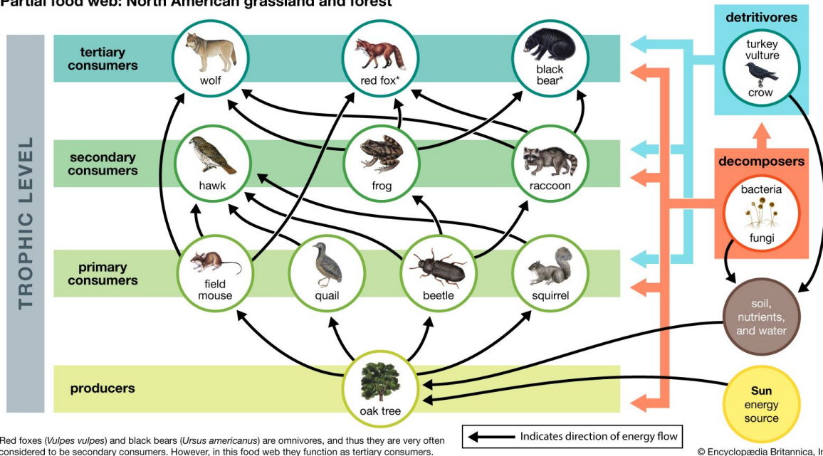
Figure 11.5: A partial food web illustrating the network of feeding relationships in a North American grassland and forest. ( Encyclopædia Britannica, Inc./Patrick O'Neill Riley )
