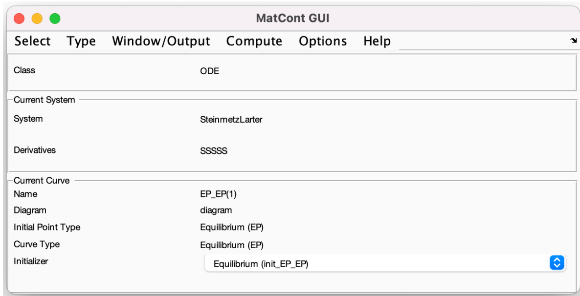
Figure 11.4: The MatCont interface.
