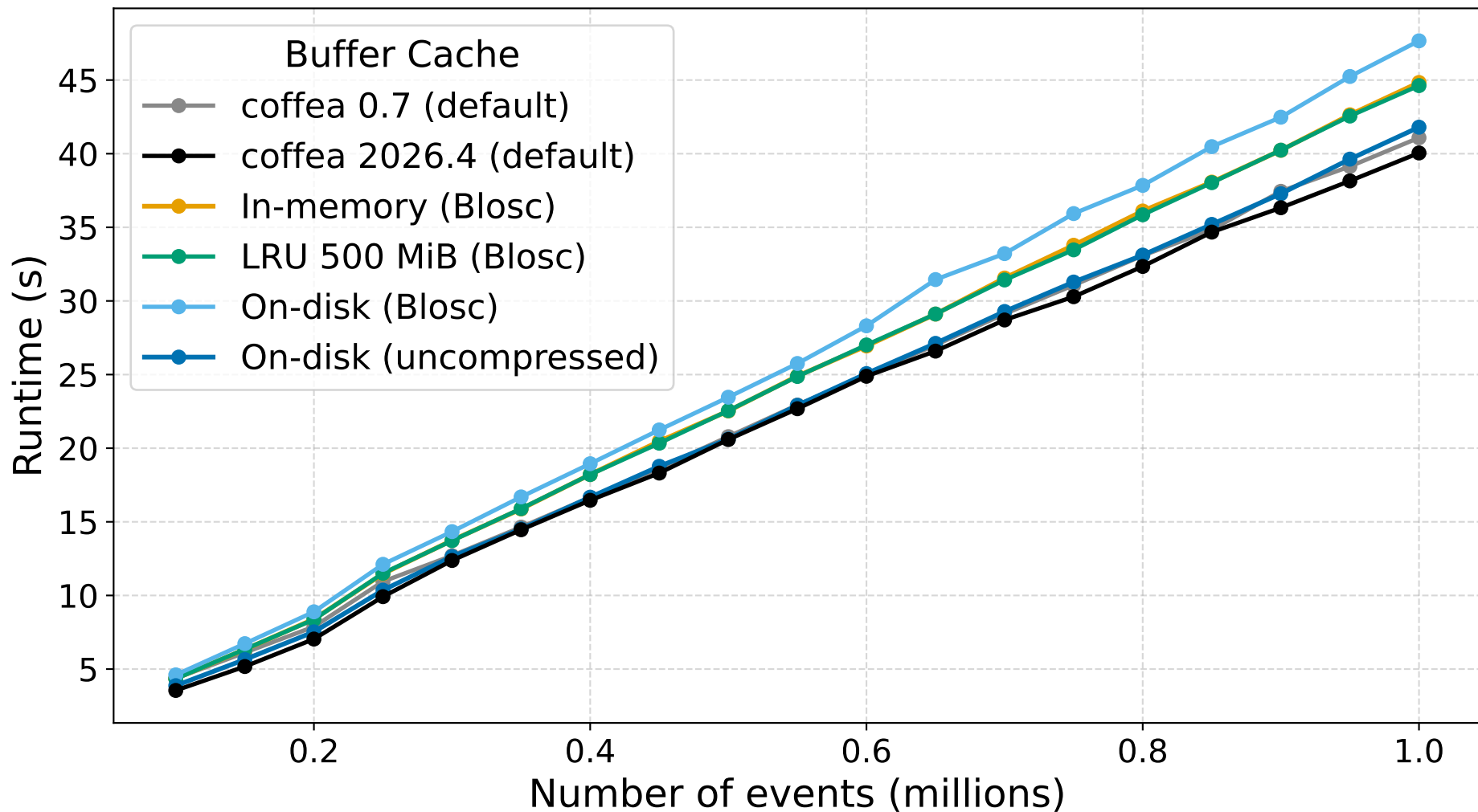
Runtime vs Number of Events
