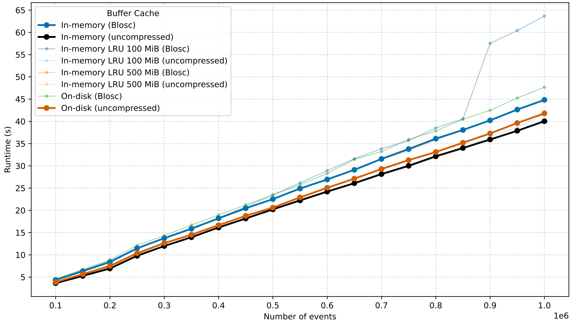
Runtime vs Number of Events
