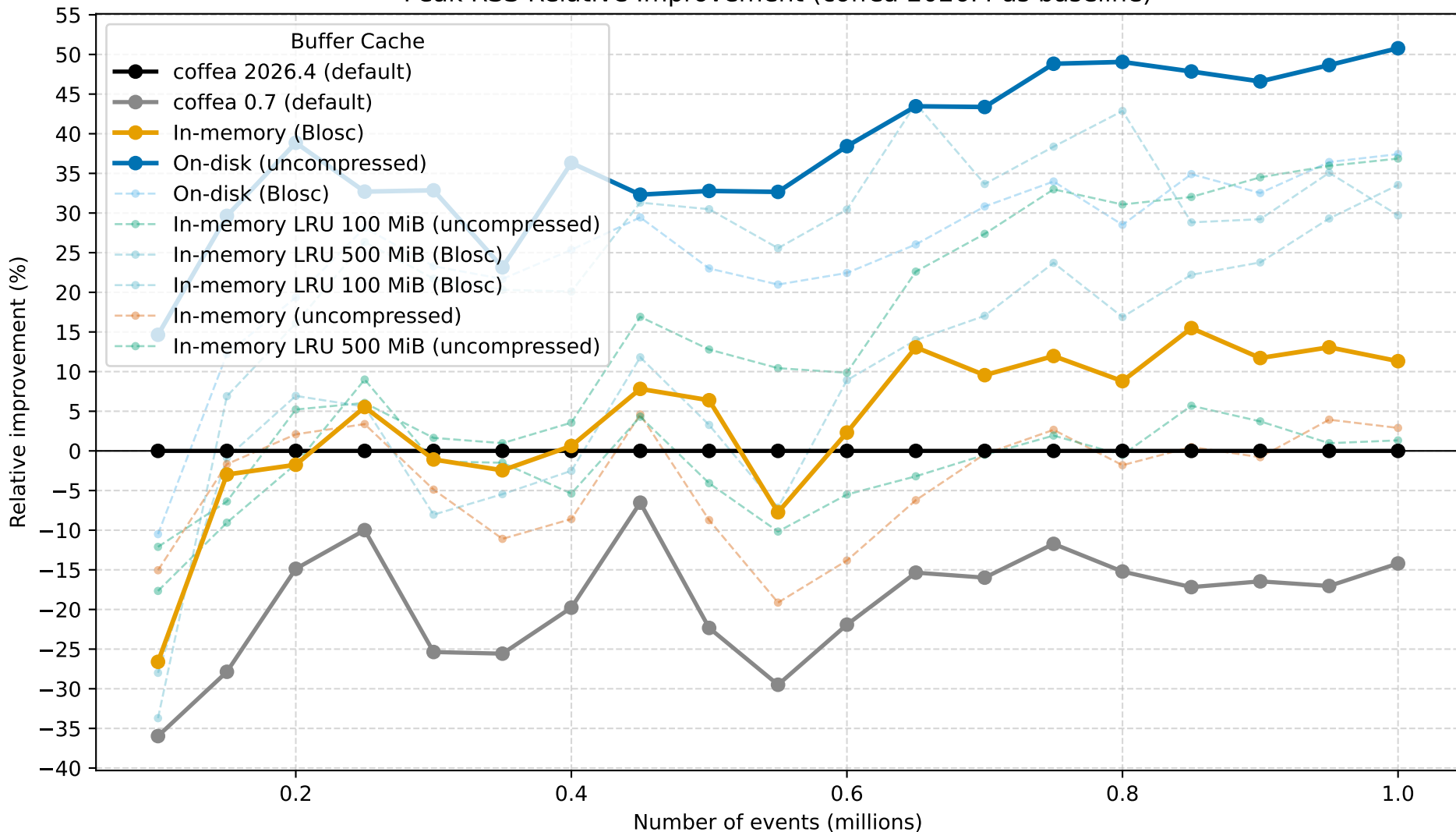
Peak RSS Relative Improvement (coffea 2026.4 as baseline)
