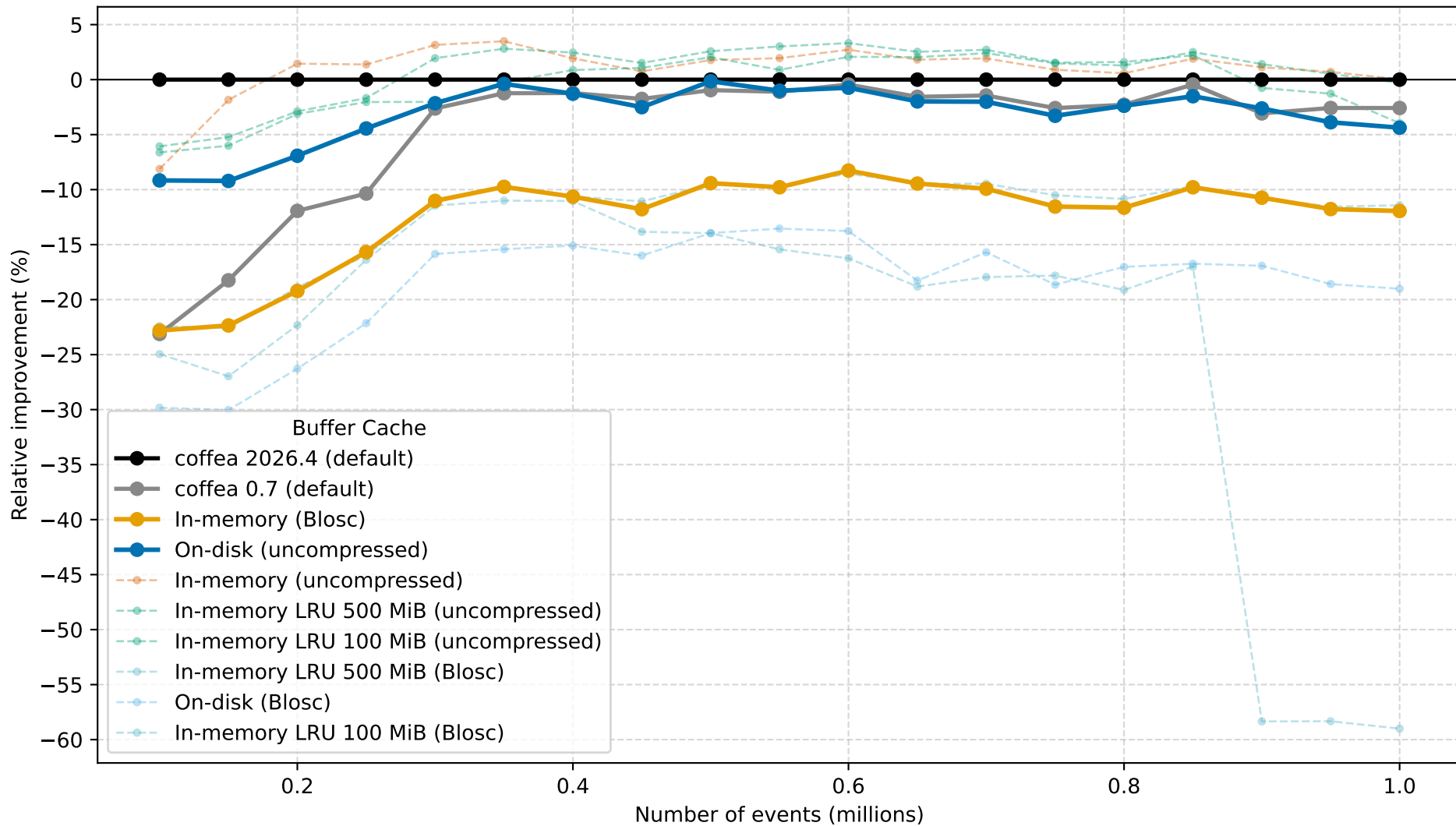
Runtime Relative Improvement (coffea 2026.4 as baseline)
