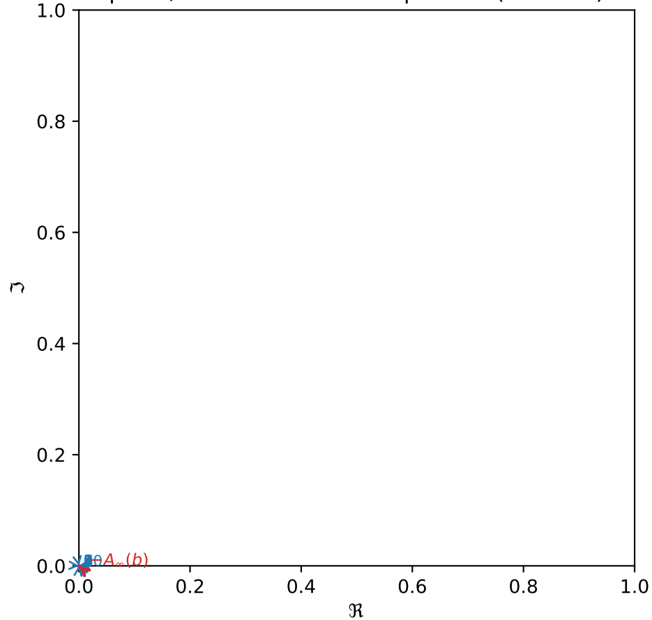
p = 3/10 : cone C -- NOT pointed (D2 false)
