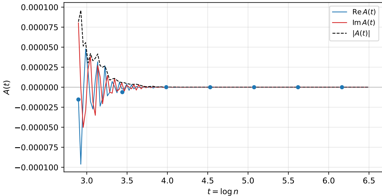
Local fundamental coefficient, p = 21/50 (dots: t_0 + kL )
