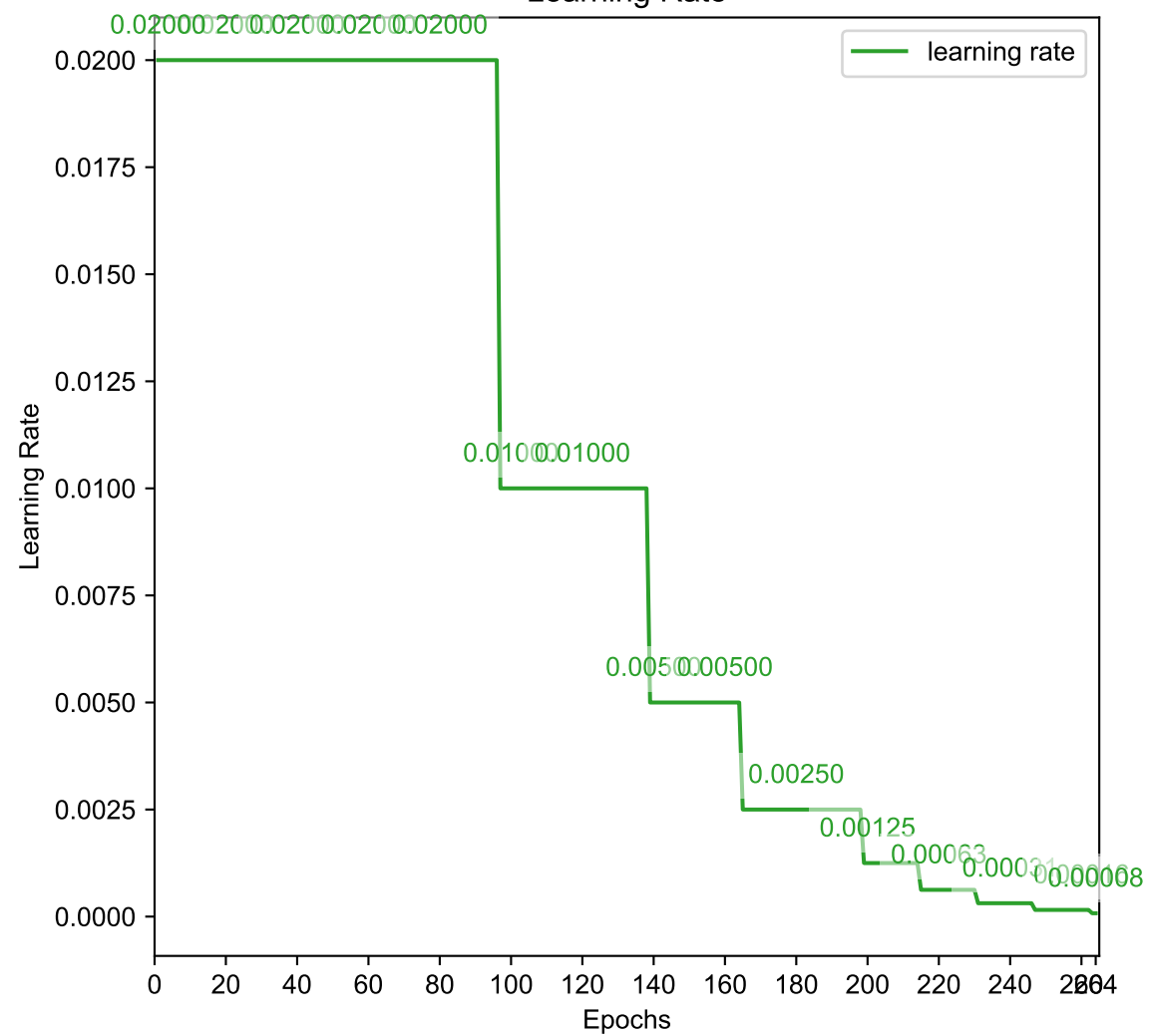
Learning Rate
