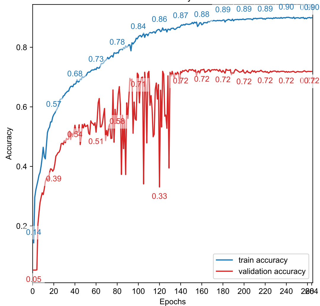
Accuracy
