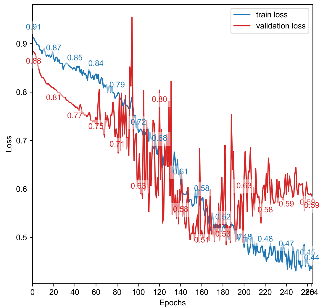
Loss
