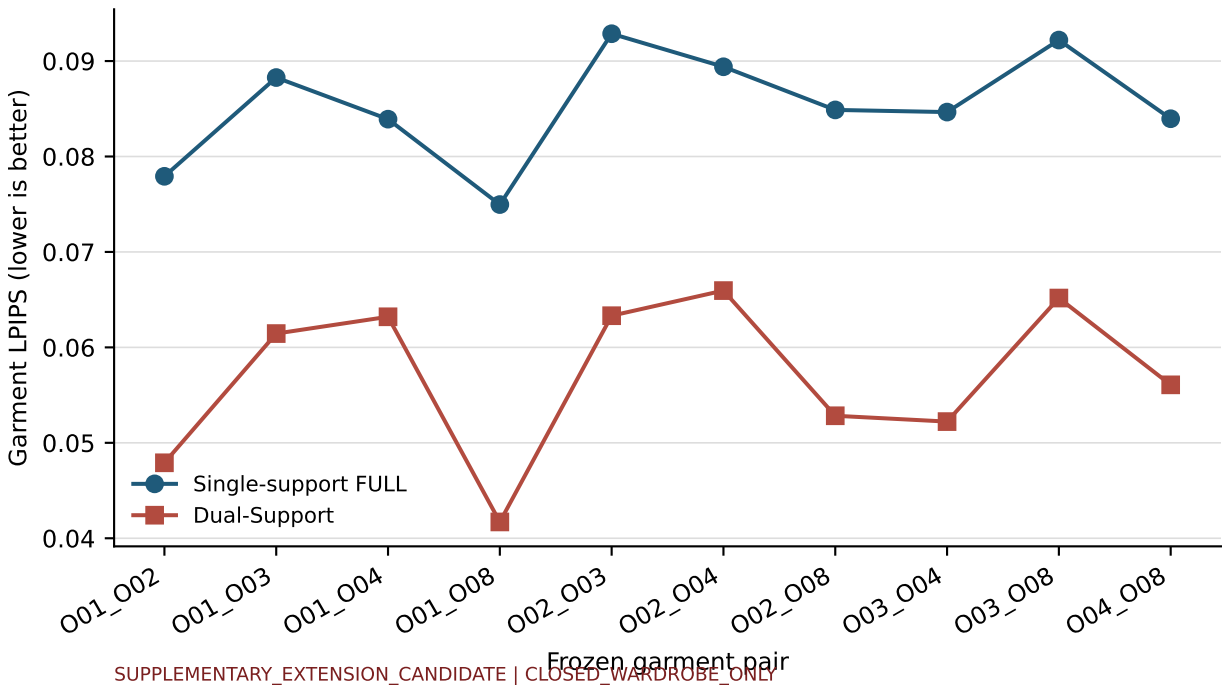
Dual-Support all-pair garment LPIPS
