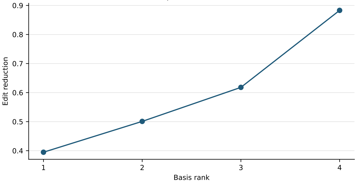
Historical explicit-basis rank ablation
