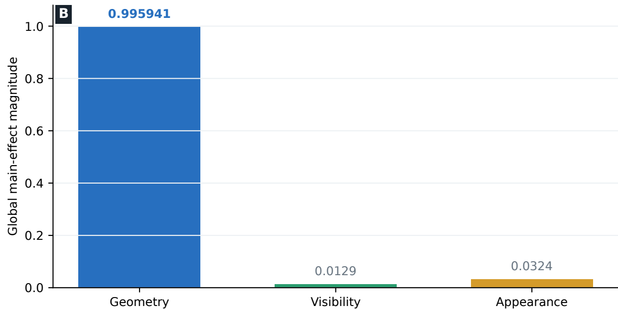
Geometry dominates all registered pair directions
