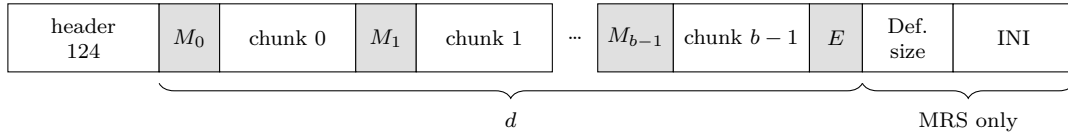
Figure 1: Container layout, not to scale. M_i is the marker of chunk i , E the end marker.
