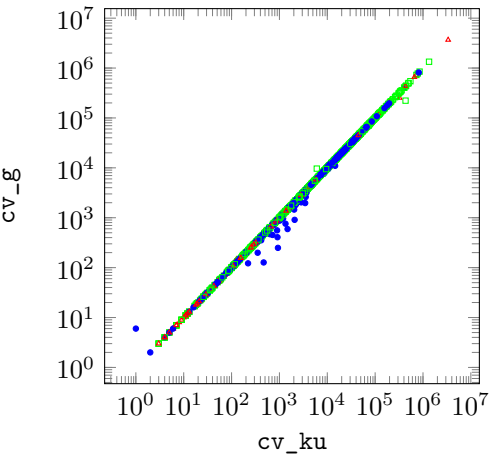
(a) k -mer counts
