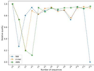
Figure 4. Comparison of the metagenomic identification quality returned by the presented method with the benchmark methods.
