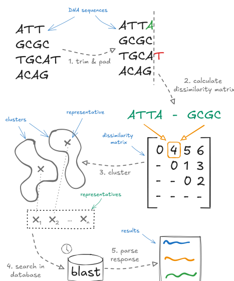
Figure 1. Overview of the pipeline: preparation of DNA sequences, dissimilarity calculation, sequence clustering, database search and postprocessing.
