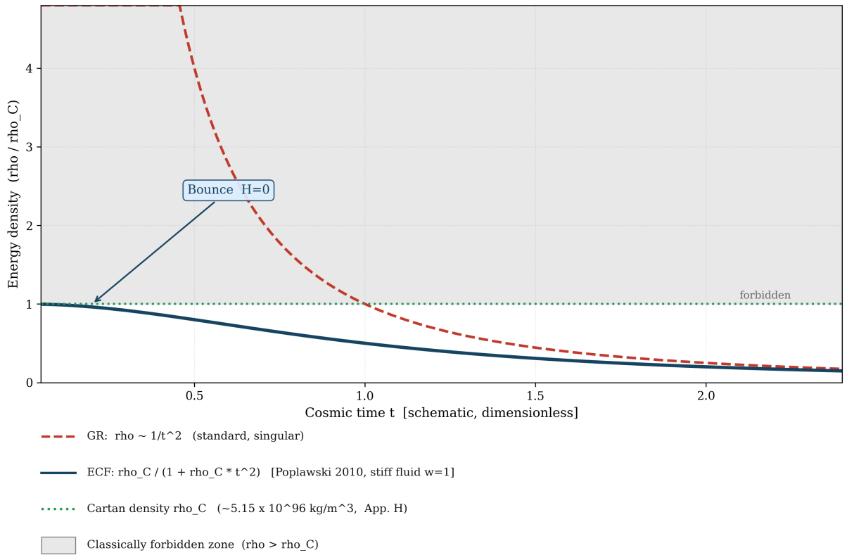
Figure 19: Regularized high-density behavior in the ECF. Illustrative comparison between the standard singular evolution and the ECF effective solution near the high-density limit. In the ECF case, the energy density approaches a finite critical value and the scale factor reaches a non-zero minimum, consistent with a non-singular bounce interpretation.
