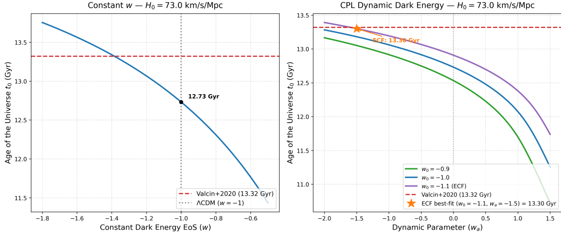
Figure 6: Phenomenological resolution of the Cosmic Age Tension through dynamical dark energy. The integration of the cosmic time t_0 is shown for an ECF-optimised expansion rate ( H_0 = 73.04 \text{ km s}^{-1} \text{ Mpc}^{-1} ) against varying equations of state. The dashed red line marks the 13.32 Gyr constraint from the oldest globular clusters [25]. Left: Under a strict cosmological constant ( w = -1 ), the universe exhibits an age deficit ( t_0 \approx 12.75 \text{ Gyr} ). Right: Relaxing the strict \Lambda assumption in favour of a CPL parameterization w(a) = w_0 + w_a(1 - a) demonstrates that a mildly phantom-crossing state ( w_0 \approx -1.1 , w_a \approx -1.5 ) can stretch the expansion integral toward stellar-age compatibility. This suggests that reconciling the H_0 tension with globular-cluster chronometry requires a dynamical relaxation of the late-time dark-energy sector, which the ECF torsional background motivates but does not uniquely fix at the level of Foundation I.
