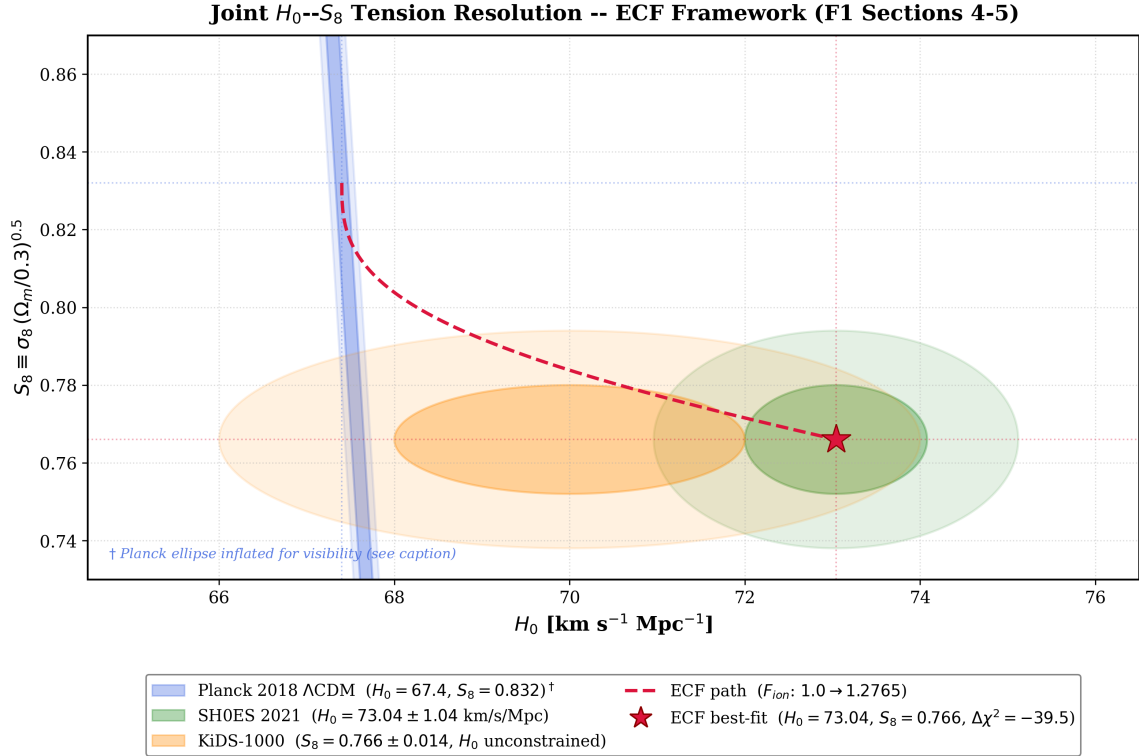
Figure 3: Joint phenomenological target in the H_0 – S_8 plane. Blue: Planck 2018 \Lambda\text{CDM} ( H_0 = 67.4, S_8 = 0.832 ) [46]. Green: SH0ES 2021 ( H_0 = 73.04 \pm 1.04 \text{ km s}^{-1} \text{ Mpc}^{-1} ) [5]. Orange: KiDS-1000 ( S_8 = 0.766 \pm 0.014; H_0 unconstrained by weak lensing alone, centre illustrative) [19]. Crimson path: ECF trajectory parameterised by F_{\text{ion}} \in [1.0, 1.2765] (cosine profile for H_0 via r_s reduction, §3; power-law for S_8 via G_{\text{eff}} suppression). Star: ECF best-fit ( \Delta\chi^2 = -39.5 vs. \Lambda\text{CDM} , §5). Ellipses show 1\sigma and 2\sigma Gaussian approximations; figure is illustrative.
