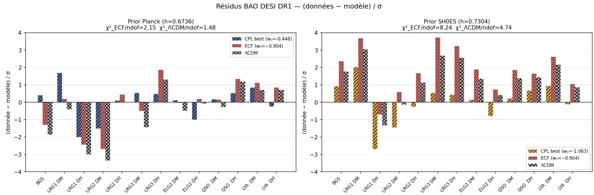
Figure 25: Normalised BAO residuals for 13 DESI DR1 observables, full covariance matrix. Each panel corresponds to one H_0 prior (Planck, SH0ES). Bars: (\text{data} - \text{model})/\sigma for CPL best-fit (hatched), ECF a priori (w_0, w_a) = (-0.904, -0.153) (dotted), and \Lambda CDM (crossed). Full covariance matrix (Adame et al. 2024 [23]); supersedes the earlier diagonal-errors figure. Reproducibility: plot_ecf_desi_mcmc_v3_0.py .
