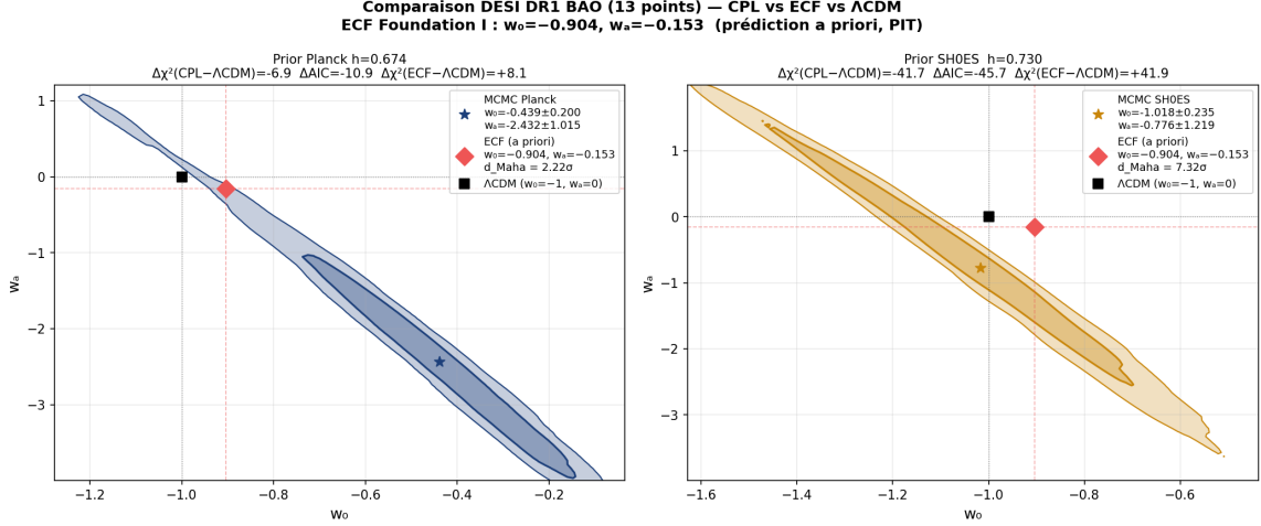
Figure 10: Independent MCMC comparison of the ECF a priori prediction with DESI DR1 BAO data (13 observables), full published covariance matrix. Filled contours: 68% and 95% marginalised posterior in the (w_0, w_a) plane for two H_0 priors. Left: Planck ( h = 0.674 ). Right: SH0ES ( h = 0.730 ) [5]. Diamond: ECF prediction (w_0, w_a) = (-0.904, -0.153) , derived from the PIT calibration prior to DESI [1]. Square: \Lambda\text{CDM} ( w_0 = -1 , w_a = 0 ). Star: MCMC median. Mahalanobis distance: d_{\text{Maha}} = 2.22\sigma (Planck), 7.32\sigma (SH0ES) — see text for the interpretation of this strong prior dependence and the \rho(w_0, w_a) \approx -0.99 degeneracy. Full covariance matrix (Adame et al. 2024 [23]); supersedes the earlier diagonal-errors figure. Reproducibility: plot_ecf_desi_mcmc_v3_0.py .
