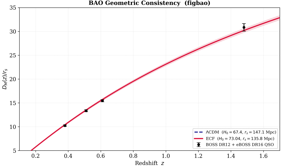
Figure 5: BAO Hubble diagram. Comparison of the ratio D_M(z)/r_s between the \Lambda CDM model and the calibrated ECF solution. The purpose of this figure is to show that the reduced sound horizon remains compatible with BAO distance measurements once the background is consistently recalibrated.
